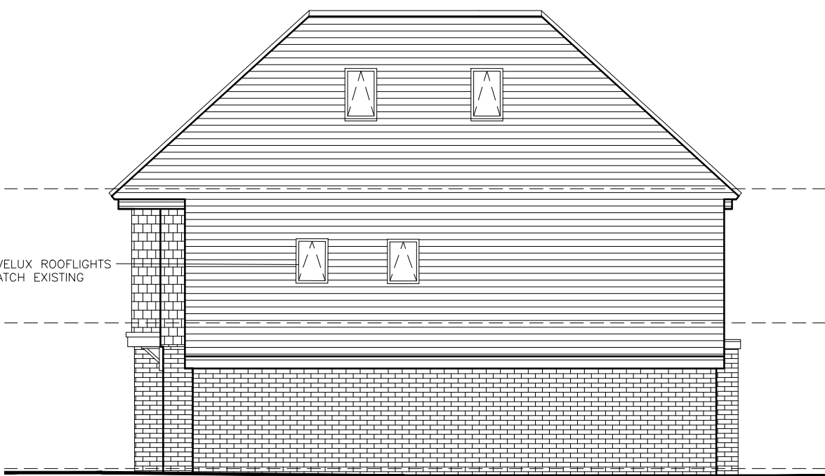
D) Proposed Side Elevation
