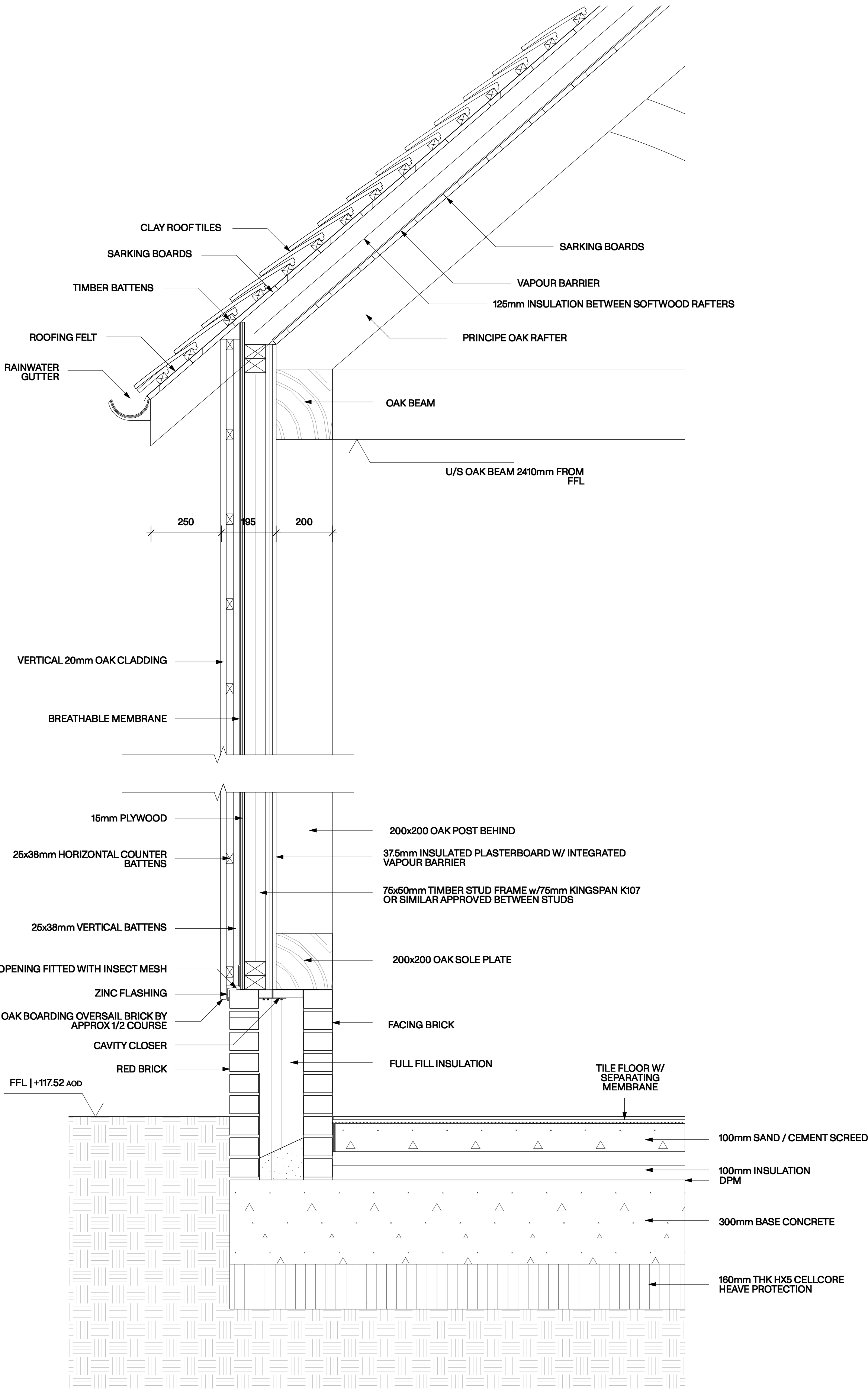
WALL DETAIL SECTION
