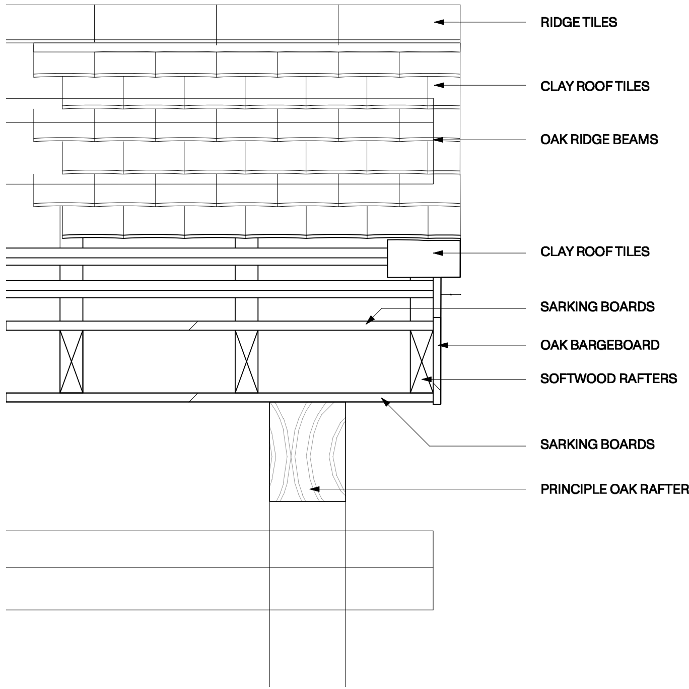
ROOF DETAIL SECTION
