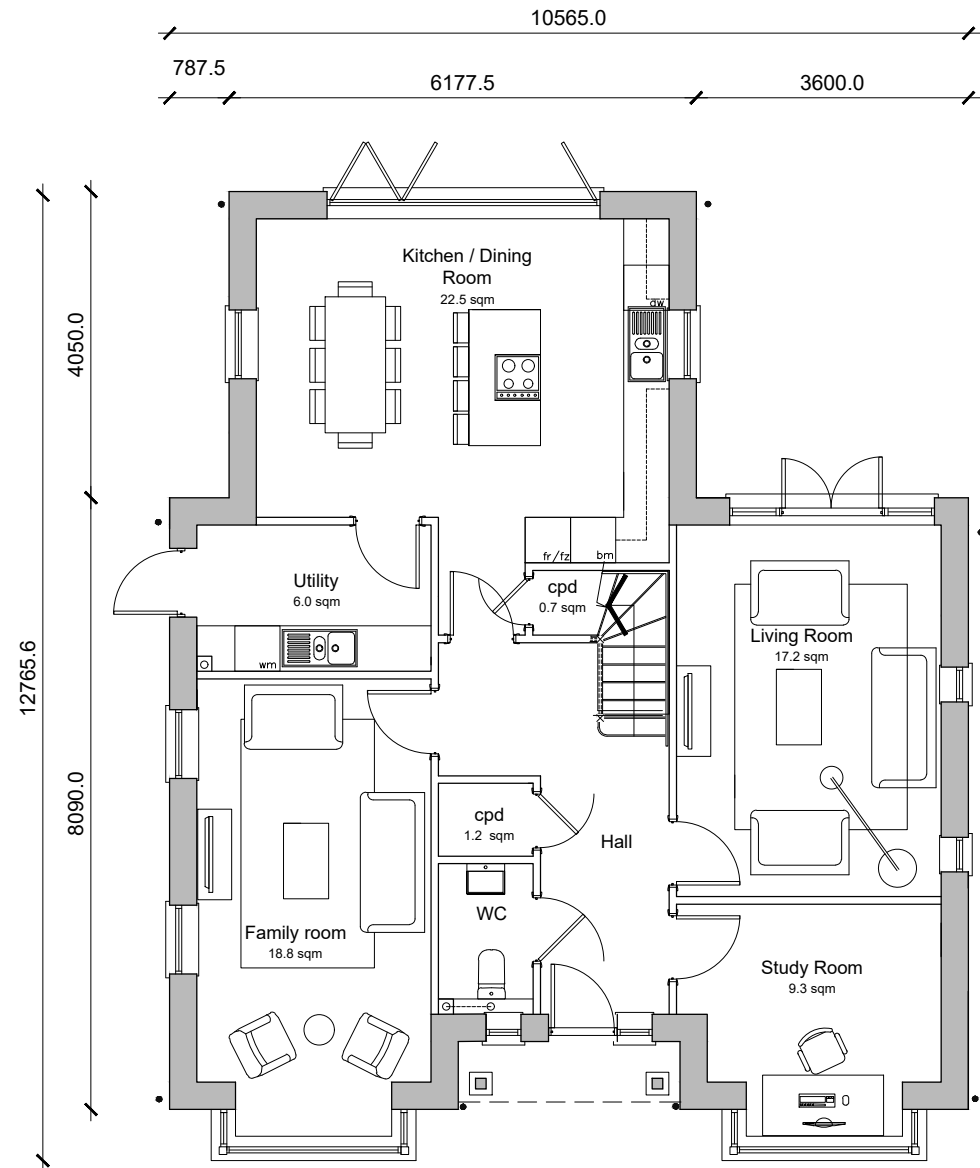
Plot 3 4-Bedroom 8-Person House 185.5m 2 / 1996 ft 2 GIA [to finishes]
