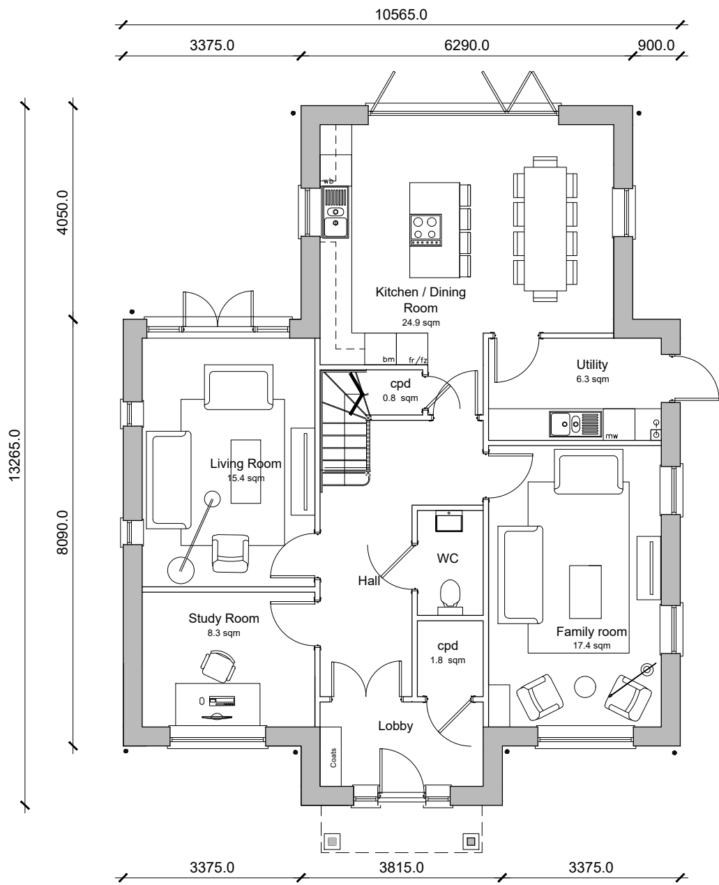
Plot 4 5-Bedroom 9-Person House 197.2m 2 / 2122 ft 2 GIA (to finishes)
