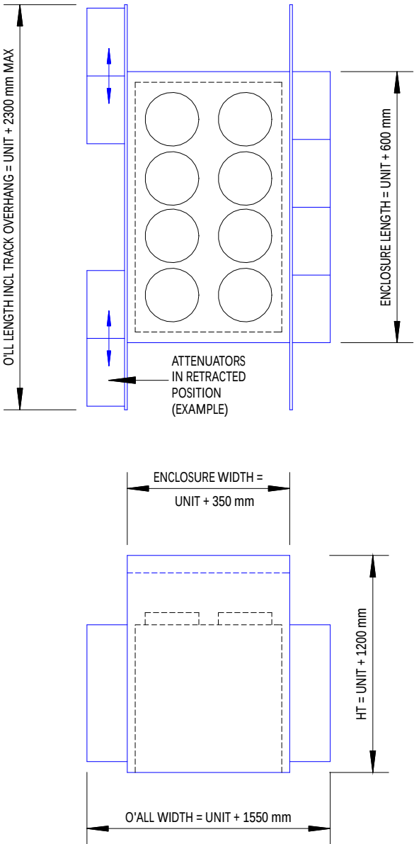
INCREASE IN DIMENSIONS OF BASE UNIT (NOMINAL)
