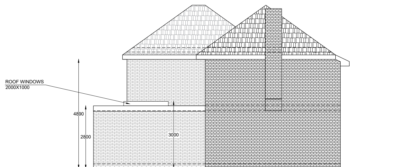
PROPOSED LEFT ELEVATION
