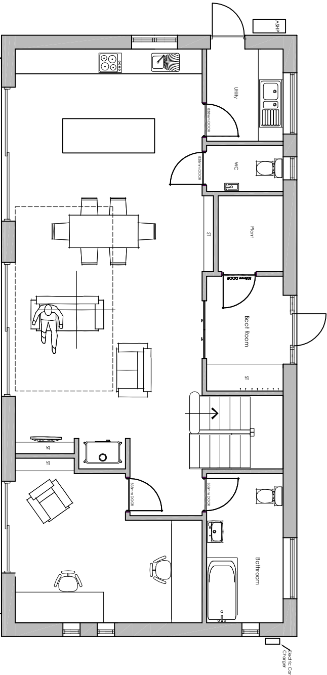
Ground Floor GIA 105 M2
