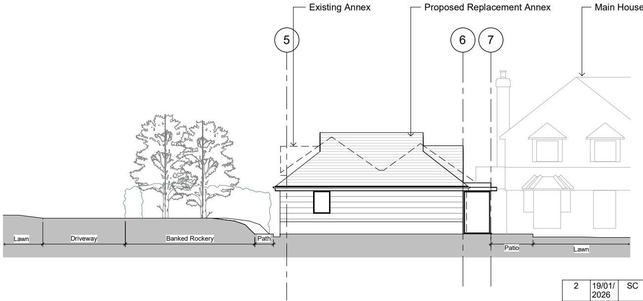
South 1 : 100
