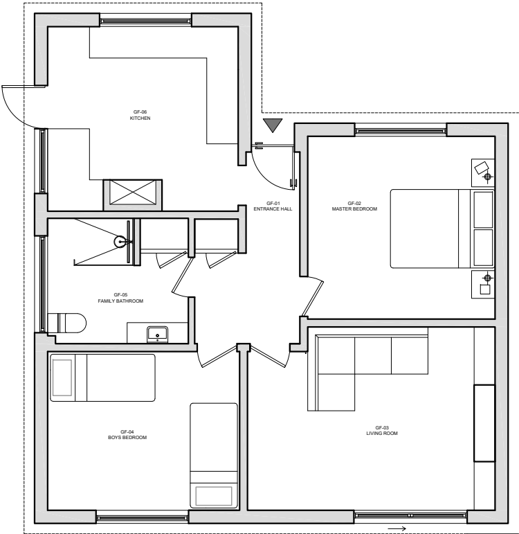
1 EXISTING 1:100 (A3) GROUND FLOOR PLAN
