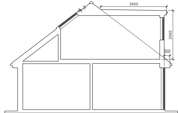
7 PROPOSED 1:100 (A3) Section AA
