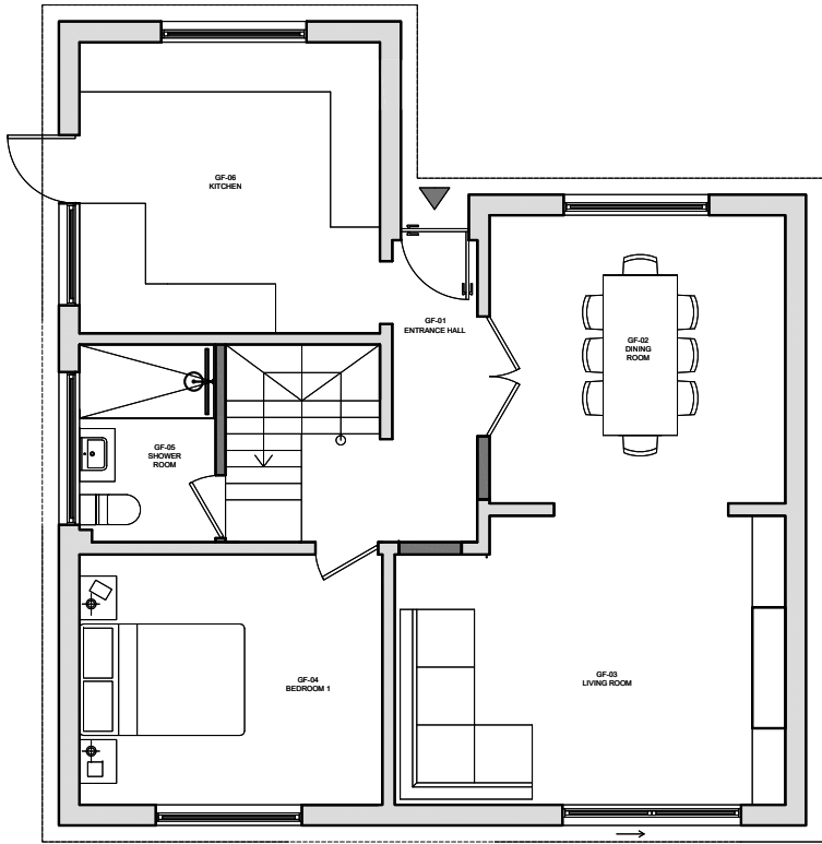
1 PROPOSED 1:100 (A3) GROUND FLOOR PLAN
