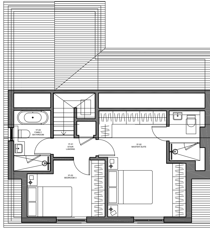
2 PROPOSED 1:100 (A3) FIRST (LOFT) FLOOR PLAN
