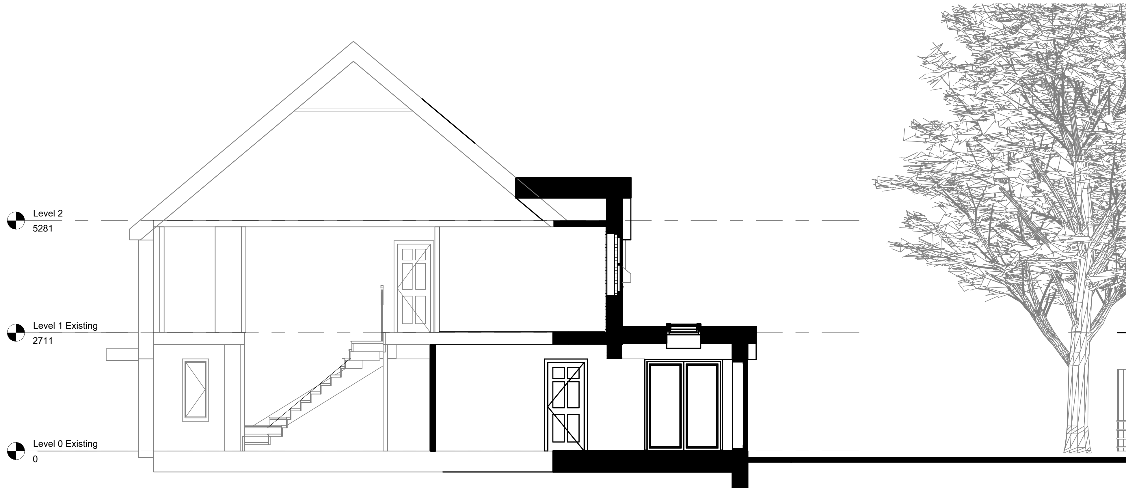
1 Proposed Section 1 1 : 50
