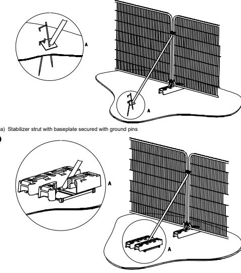
Figure 3 Examples of above-ground stabilizing systems
