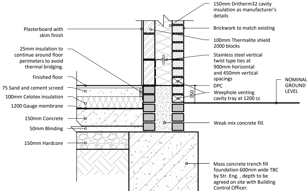
Rear Wall Foundation Scale 1/20@A3
