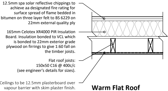
Warm Flat Roof Scale 1/20@A3
