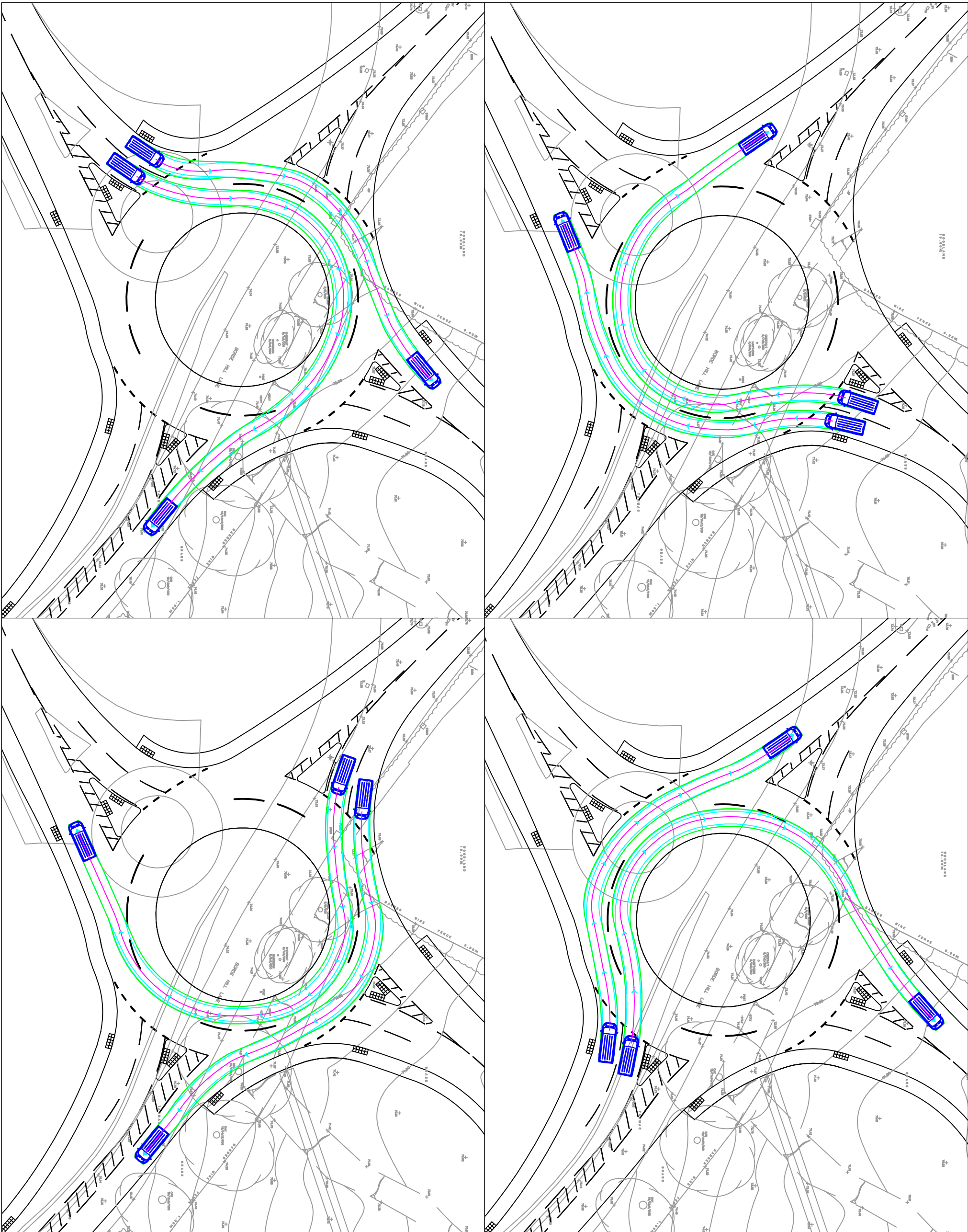
L2H3 FORD TRANSIT
