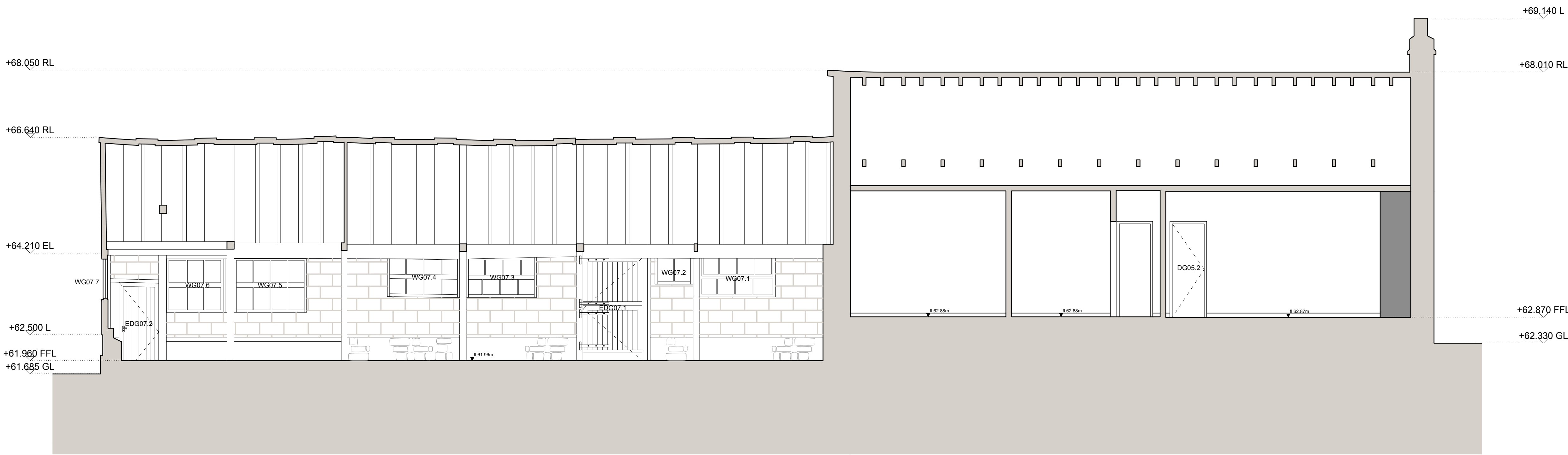
02 Stables and Cottage Existing Long Section 1:50 @ A1; 1:100 @ A3
