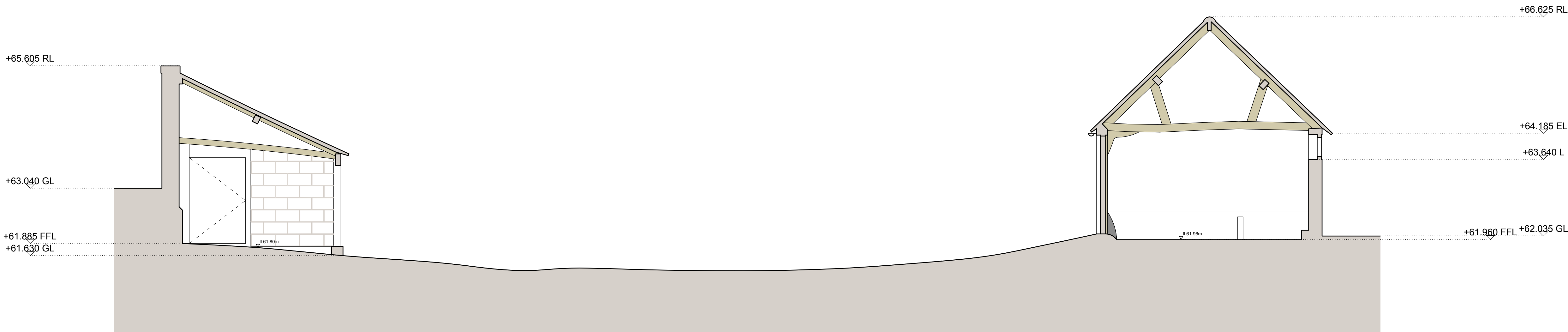
01 Byre and Stables Existing Cross Section 1:50 @ A1; 1:100 @ A3
