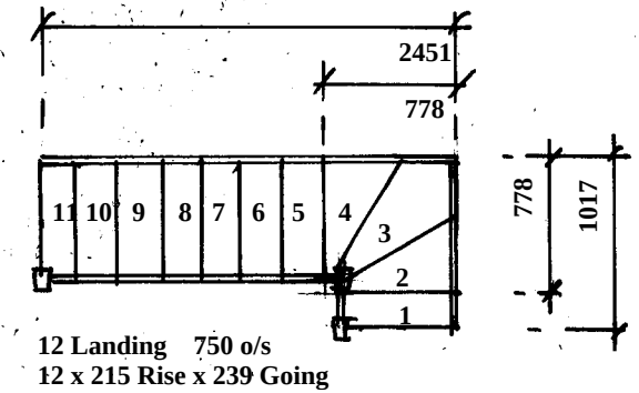
Proposed Staircase Plan
