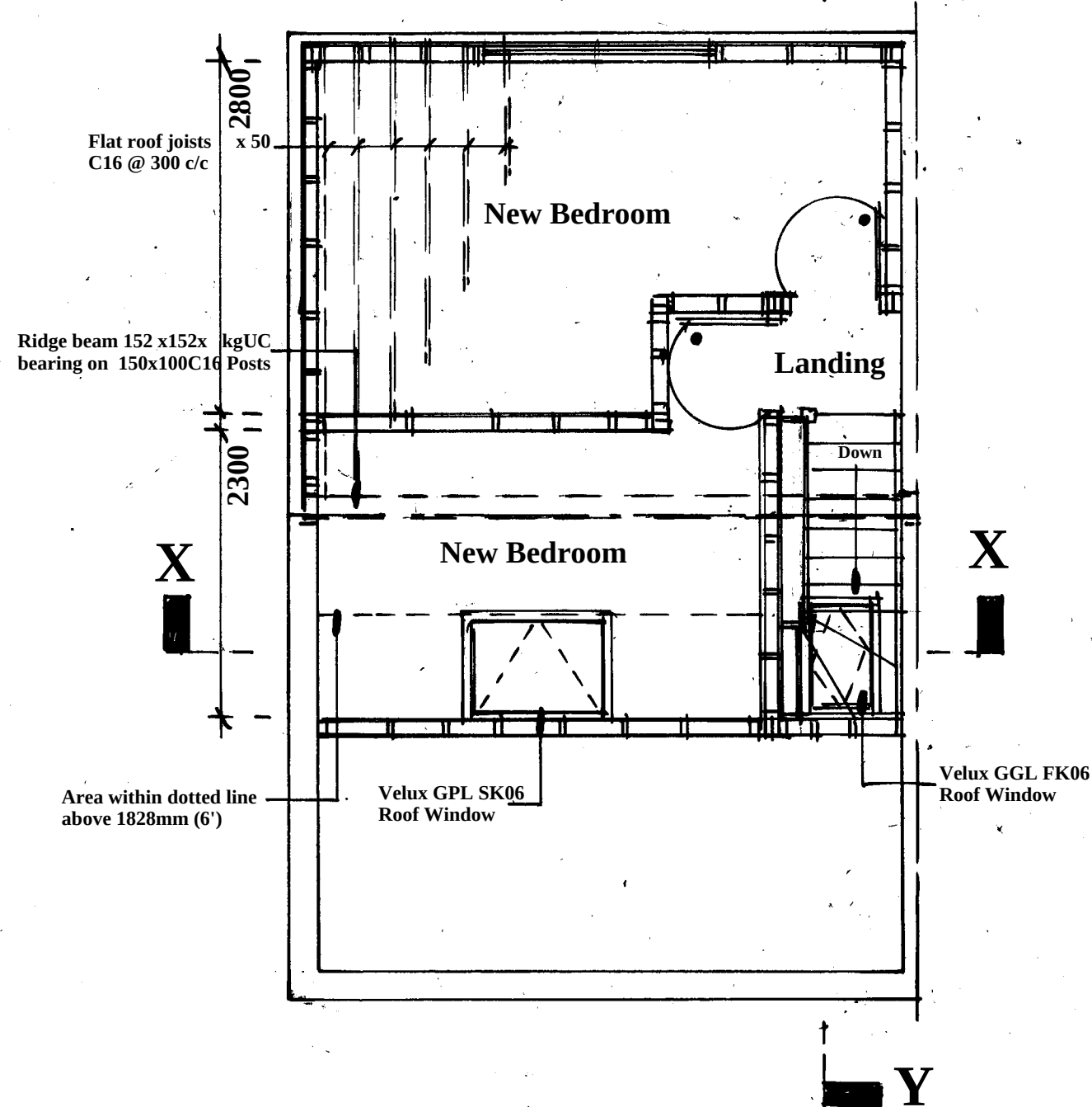
Proposed Loft Room Plan
