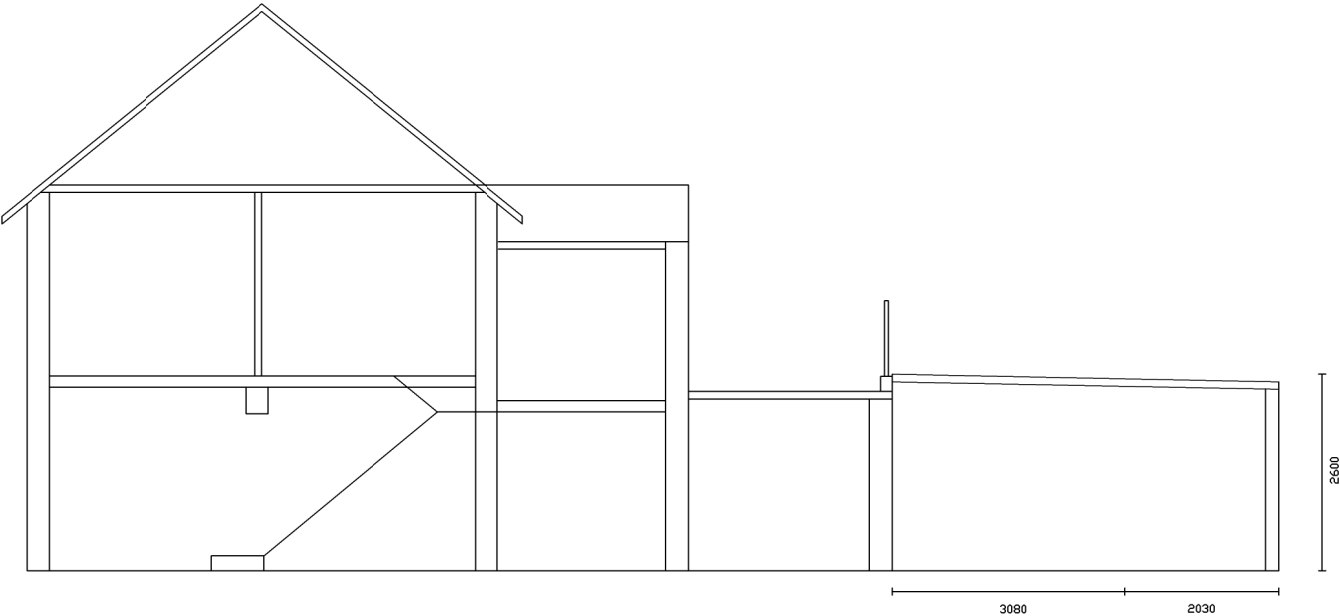
Proposed Cross Section A-A
