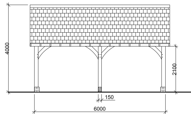
FRONT ELEVATION
