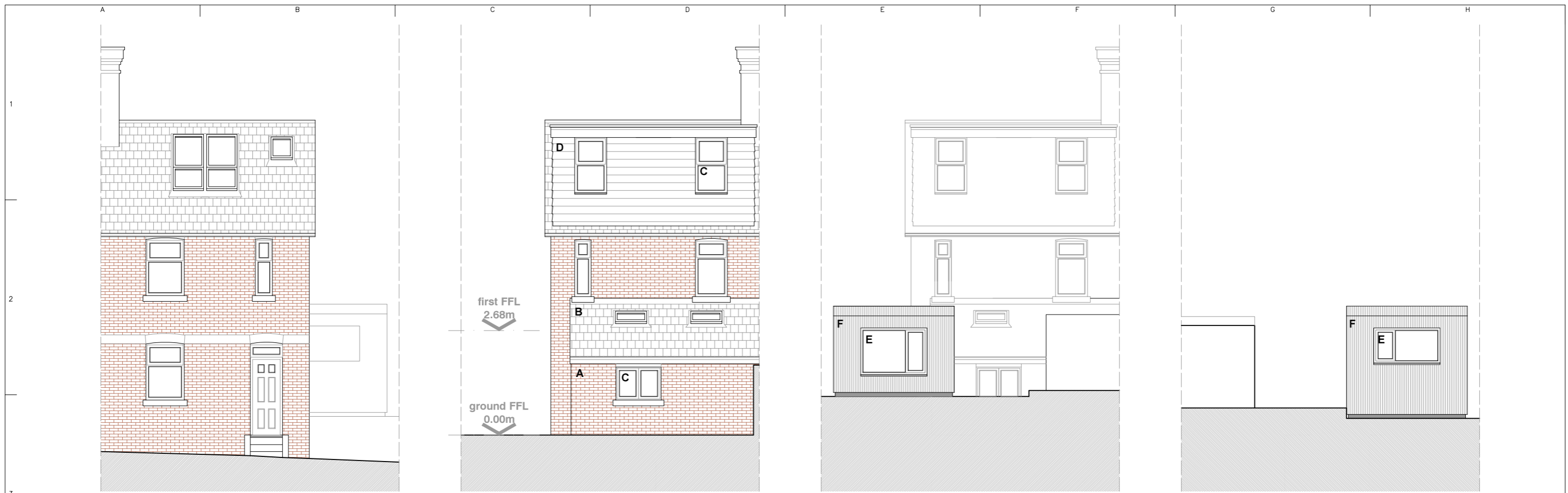
120.1 FRONT ELEVATION (west)
