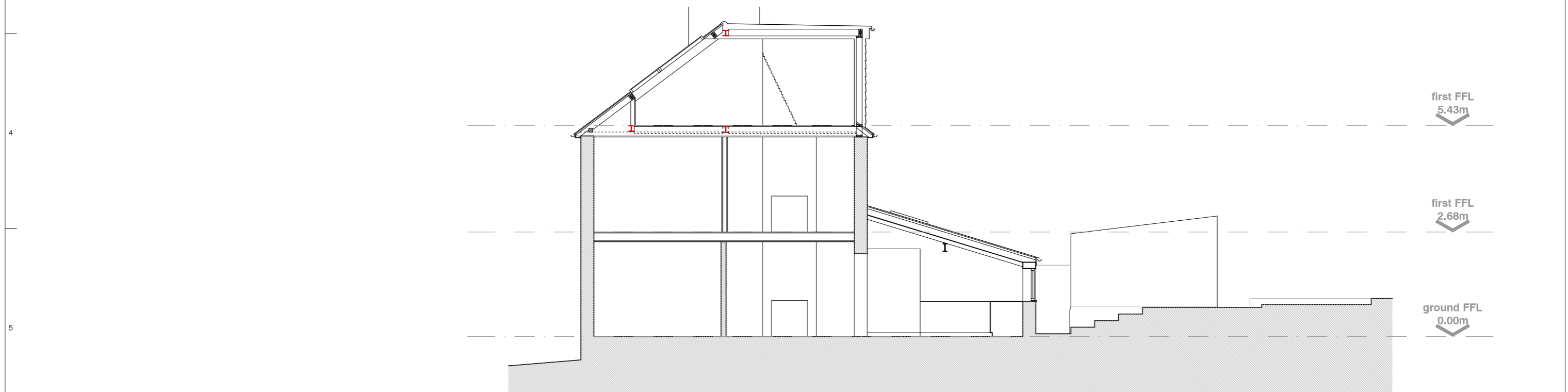
130.2 SECTION
