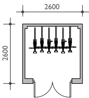
FLOOR PLAN
