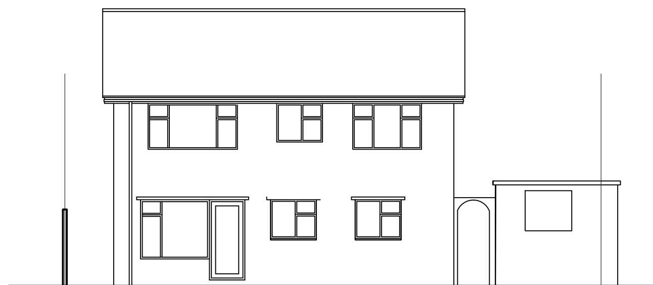
EXISTING REAR (NORTH) ELEVATION
