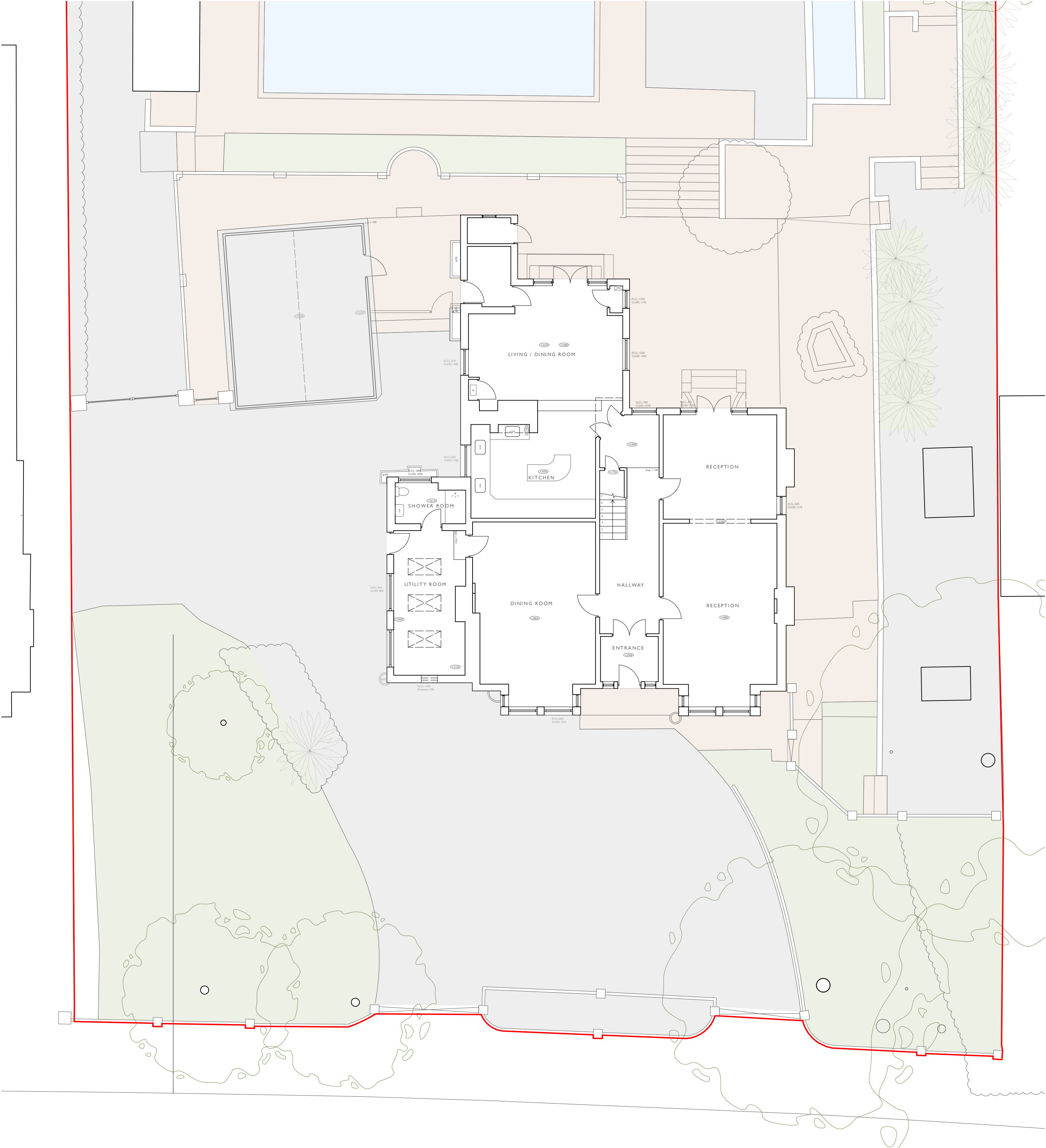
I. GROUND FLOOR
