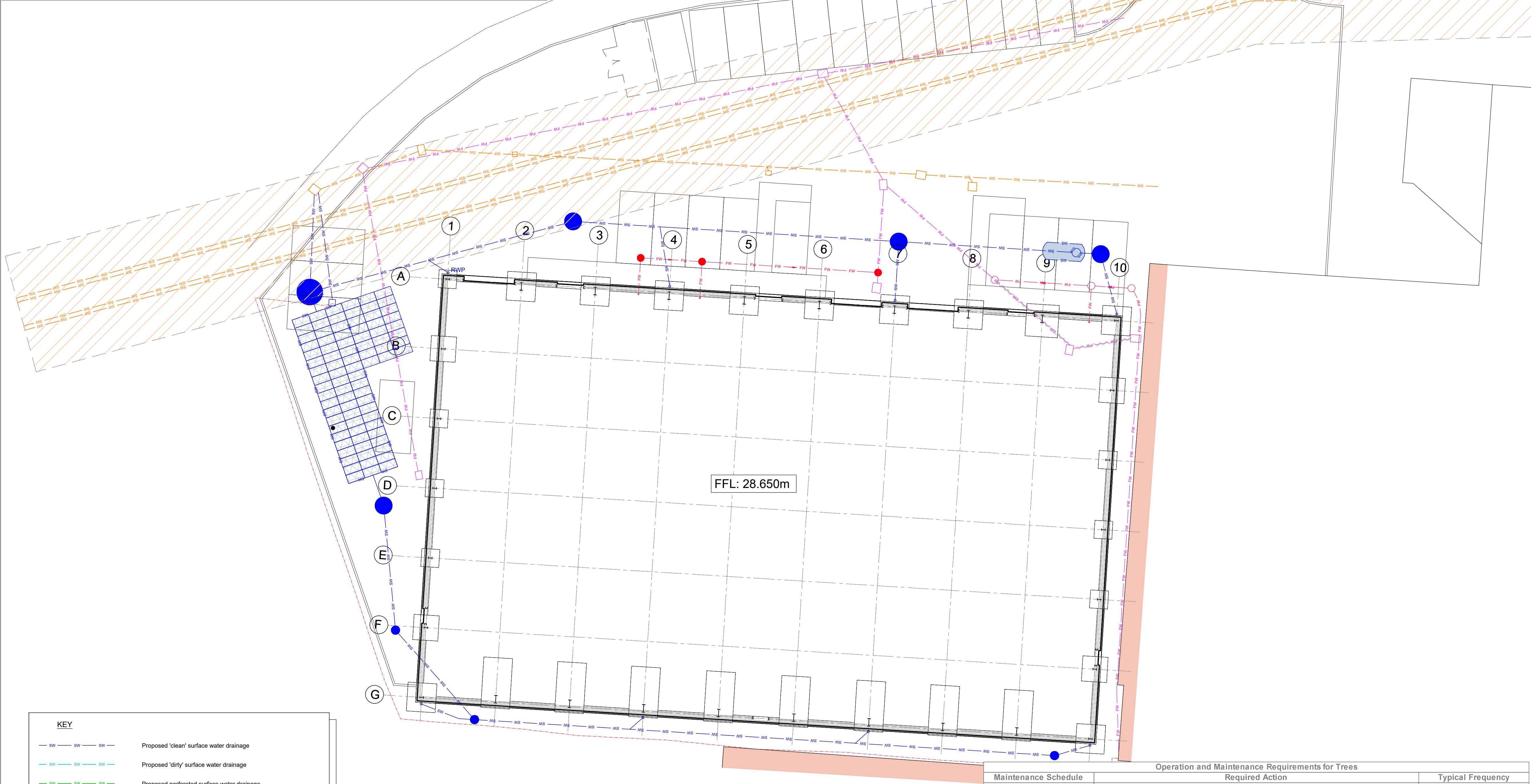
PLAN Scale 1:150
