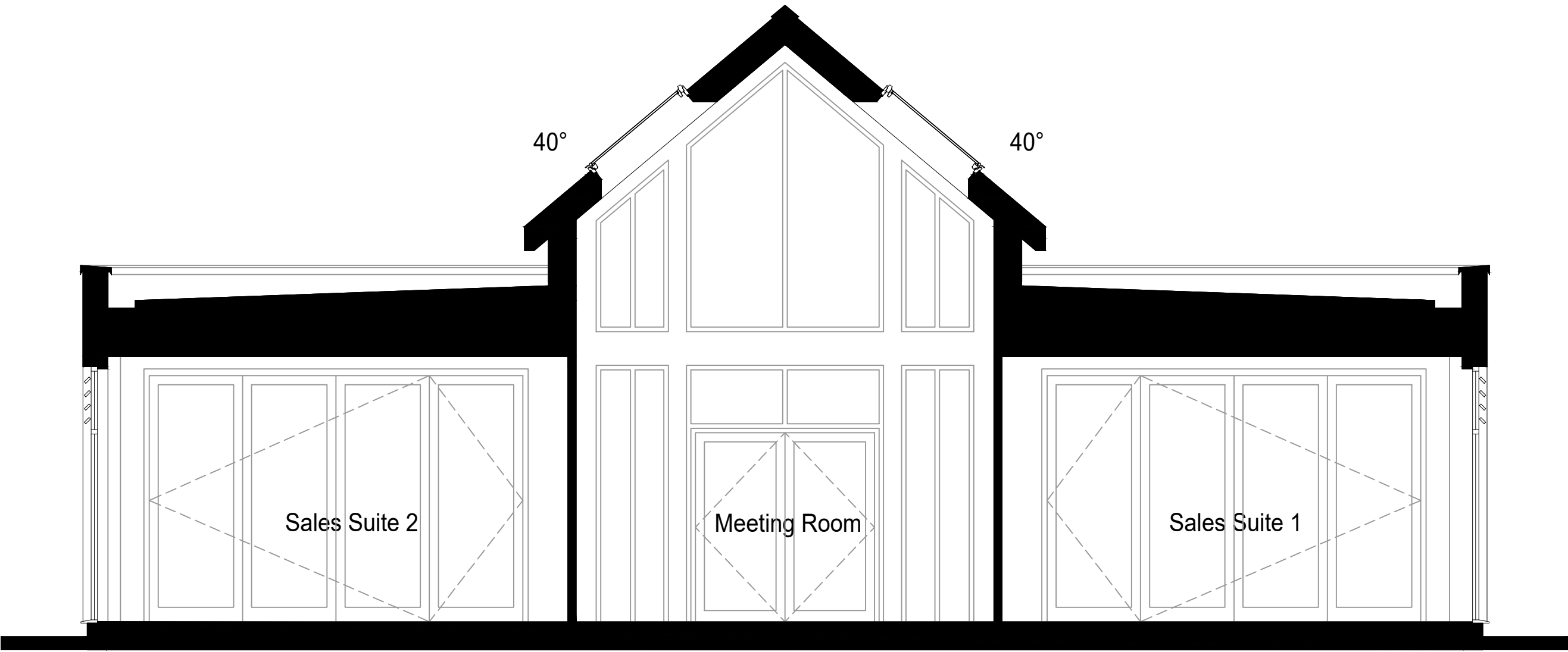
Section C-C
