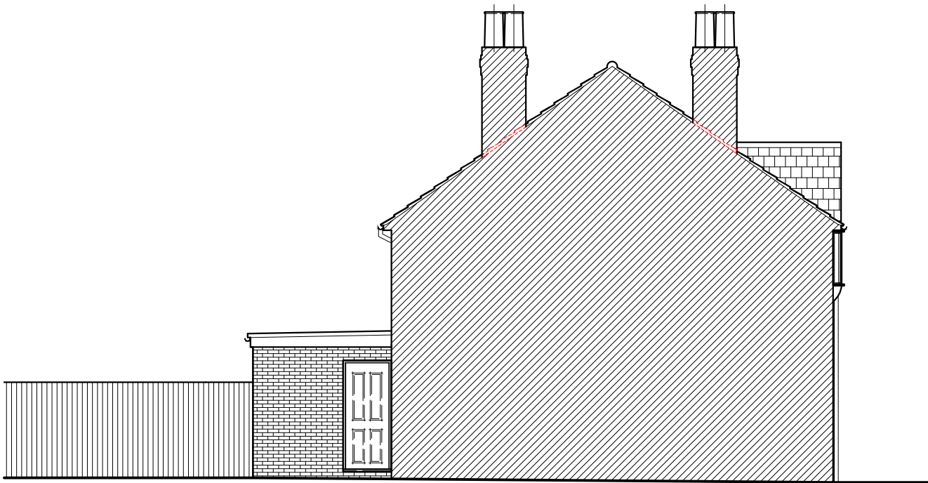
Side Elevation
