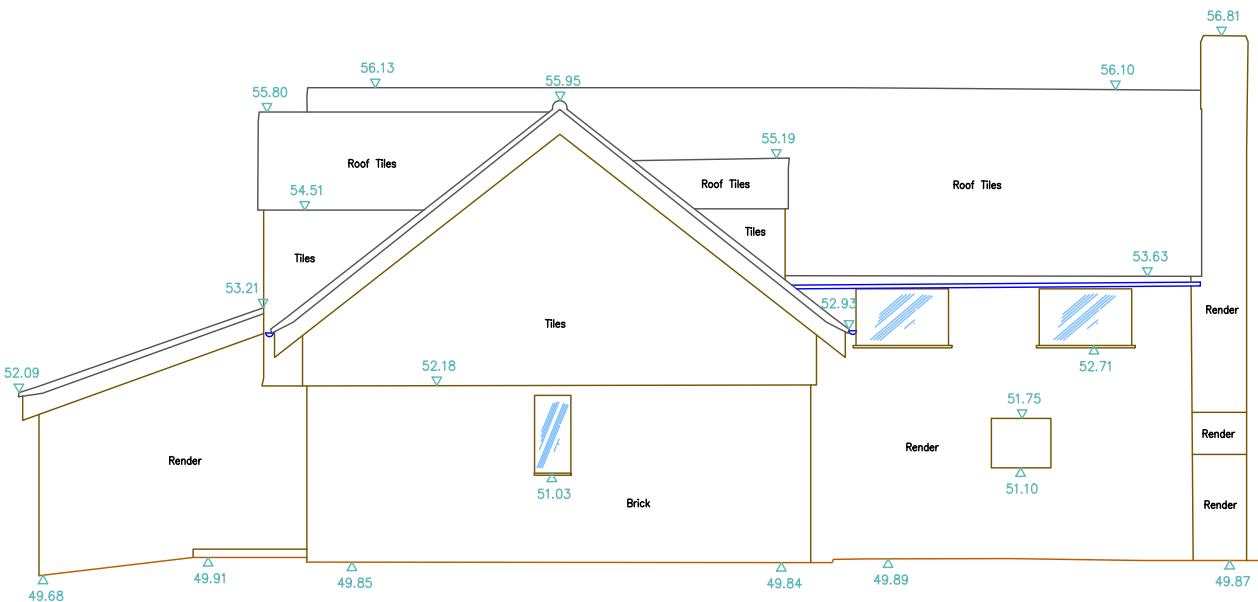
North Elevation
