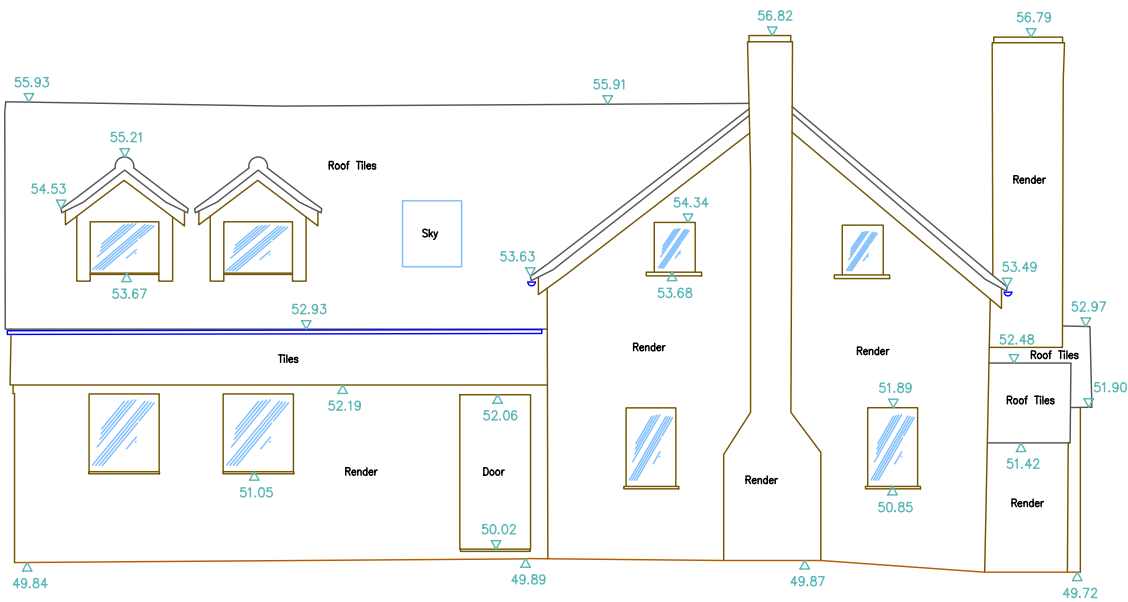
West Elevation
