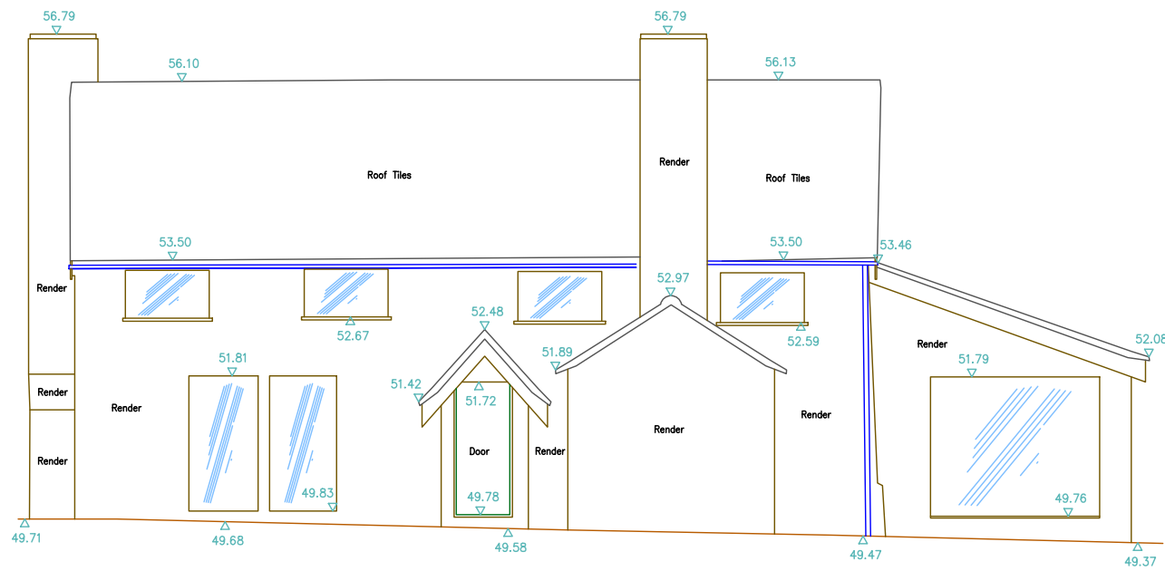
South Elevation
