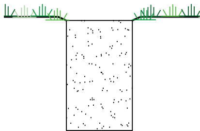
Ring beam indicative section 1:50 Depth and specification TBC by engineer.
