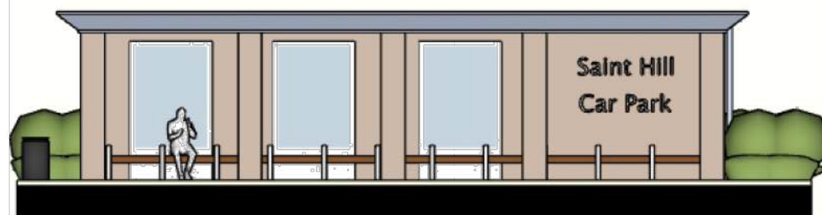
Proposed East Elevation 1:100
