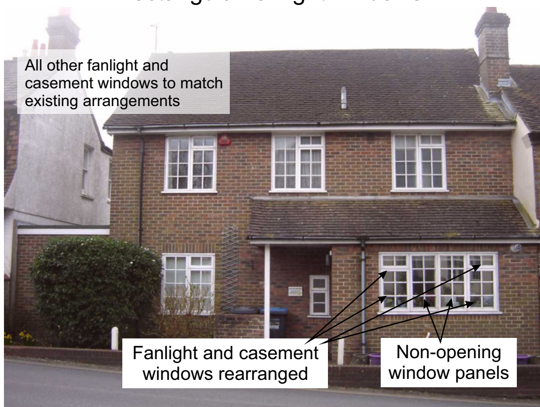
Proposed arrangement of casement and rectangular fanlight windows
