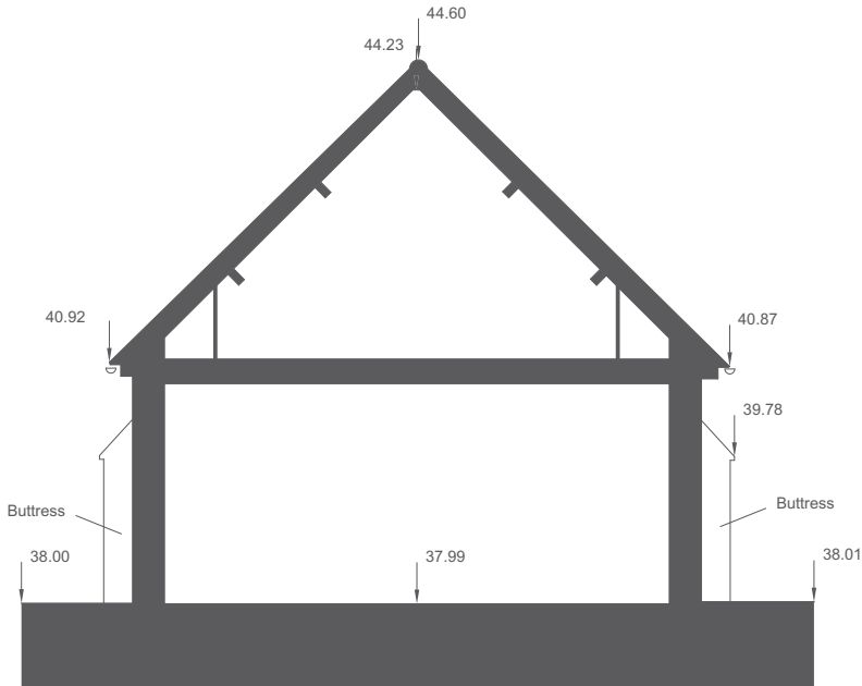
02 - PROPOSED SECTION 2
