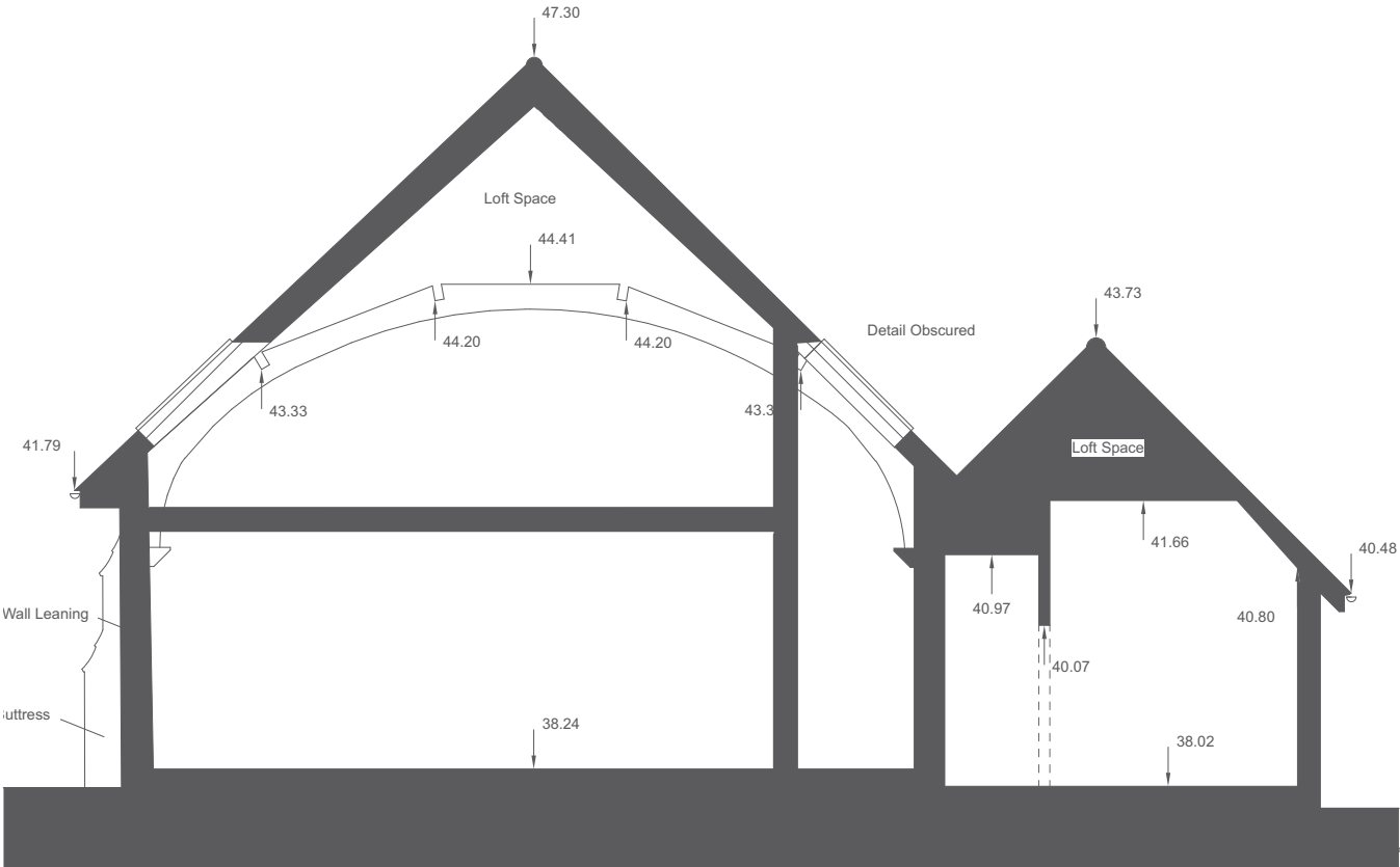
01 - PROPOSED SECTION 1
