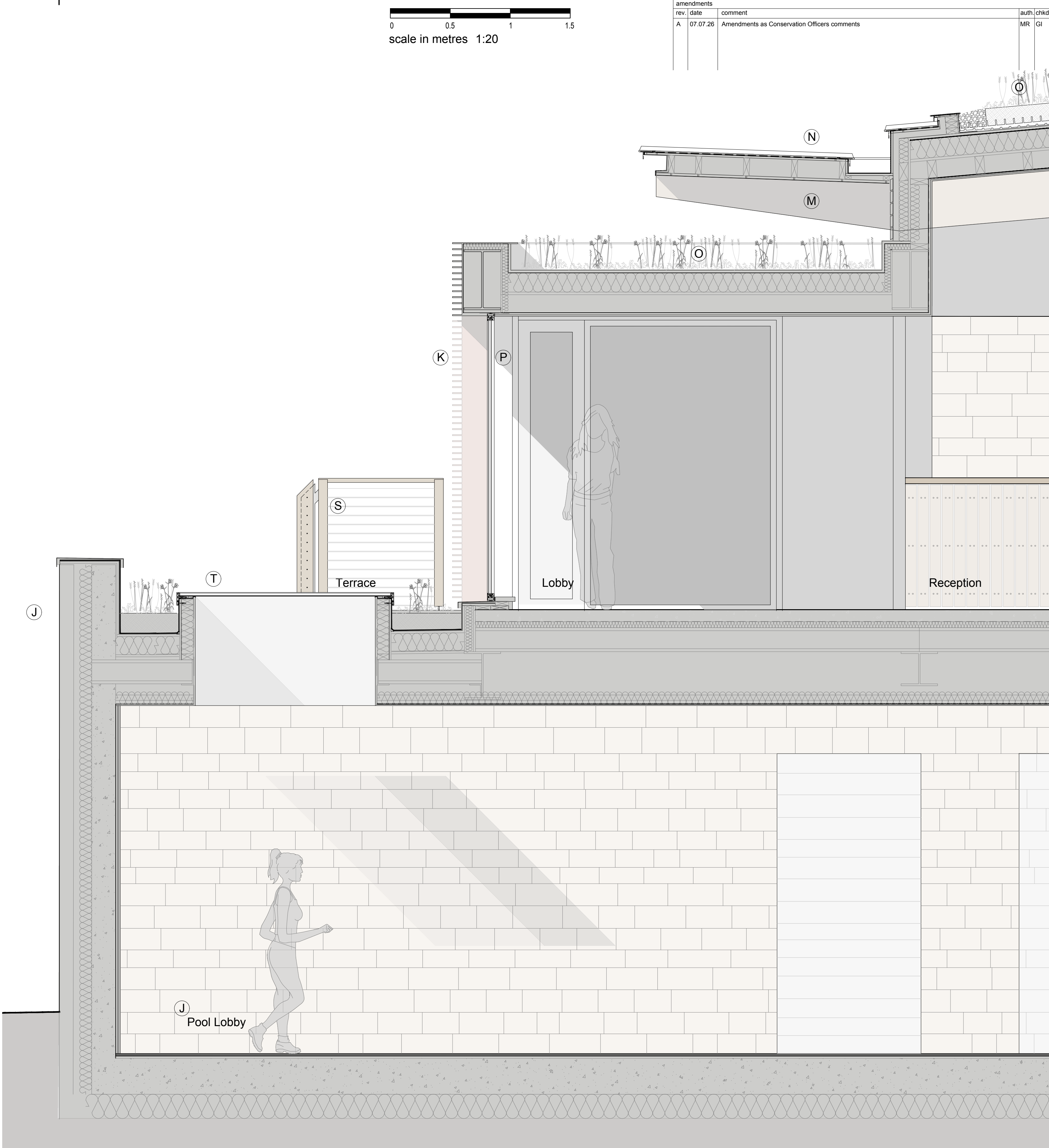
Proposed Detail Section 1:20
