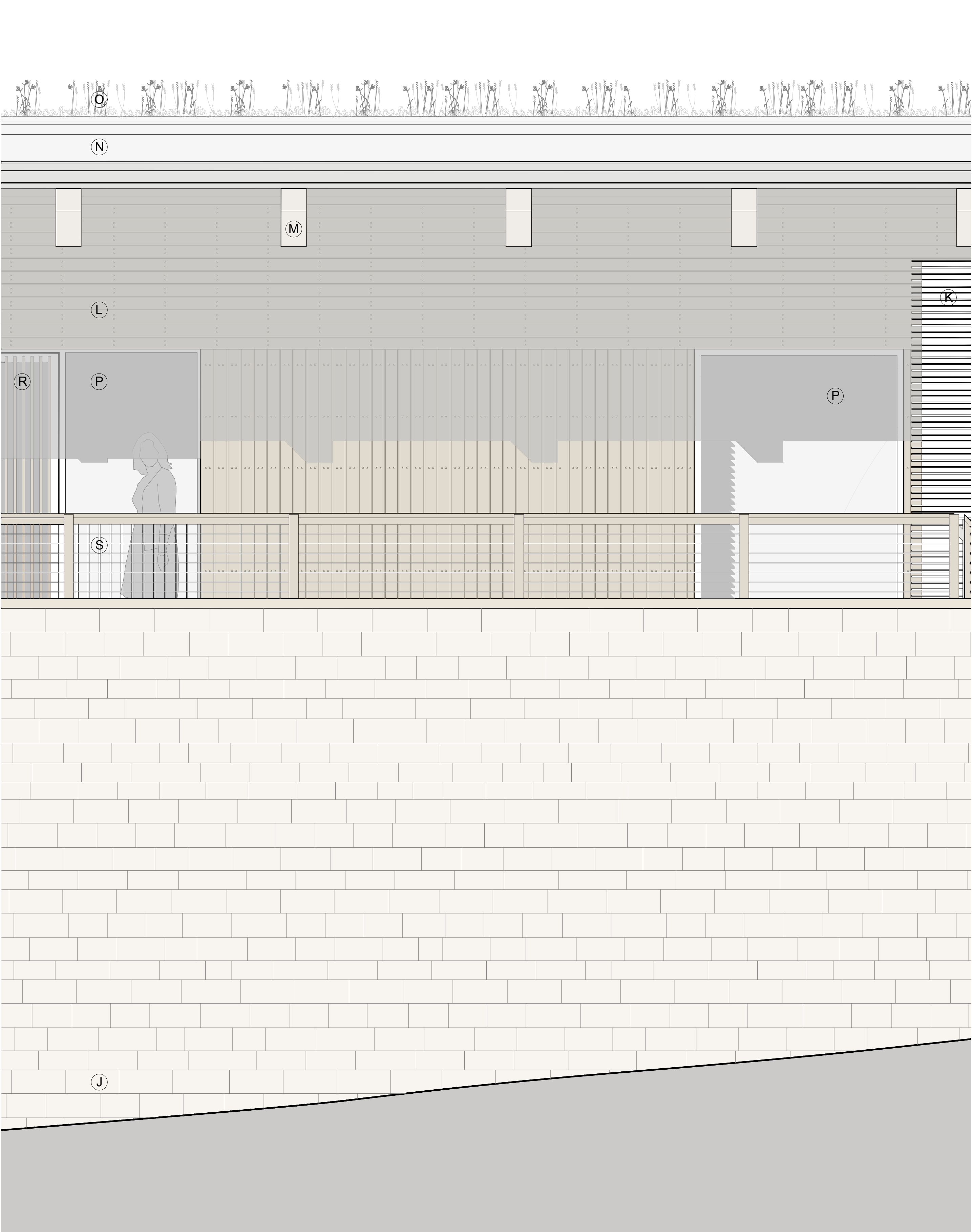
Proposed Detail Elevation 1:20
