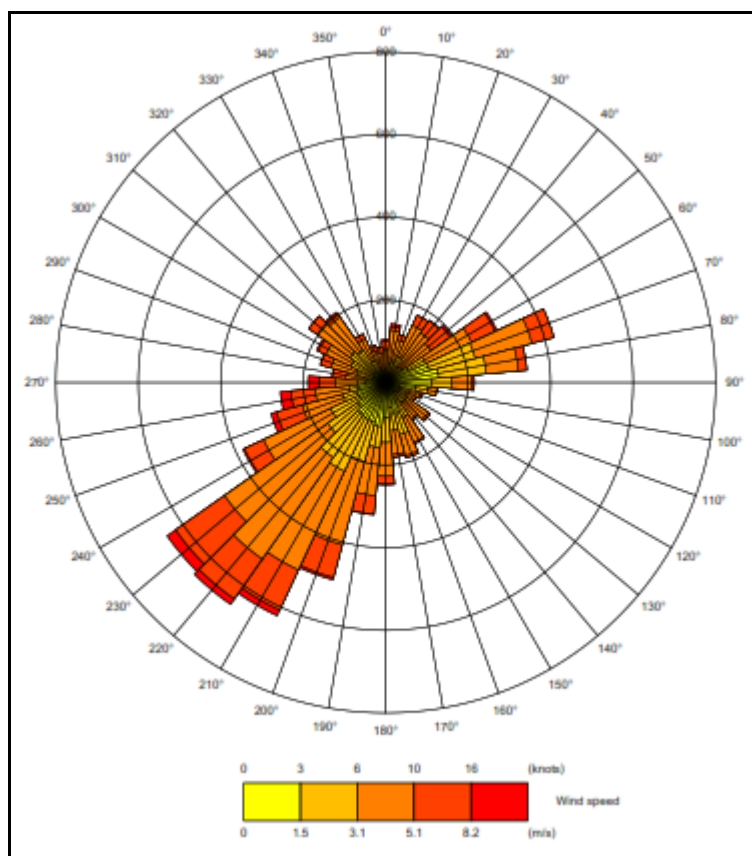
Figure 5.1: Wind Rose for Gatwick Airport Meteorological Station (2022)
