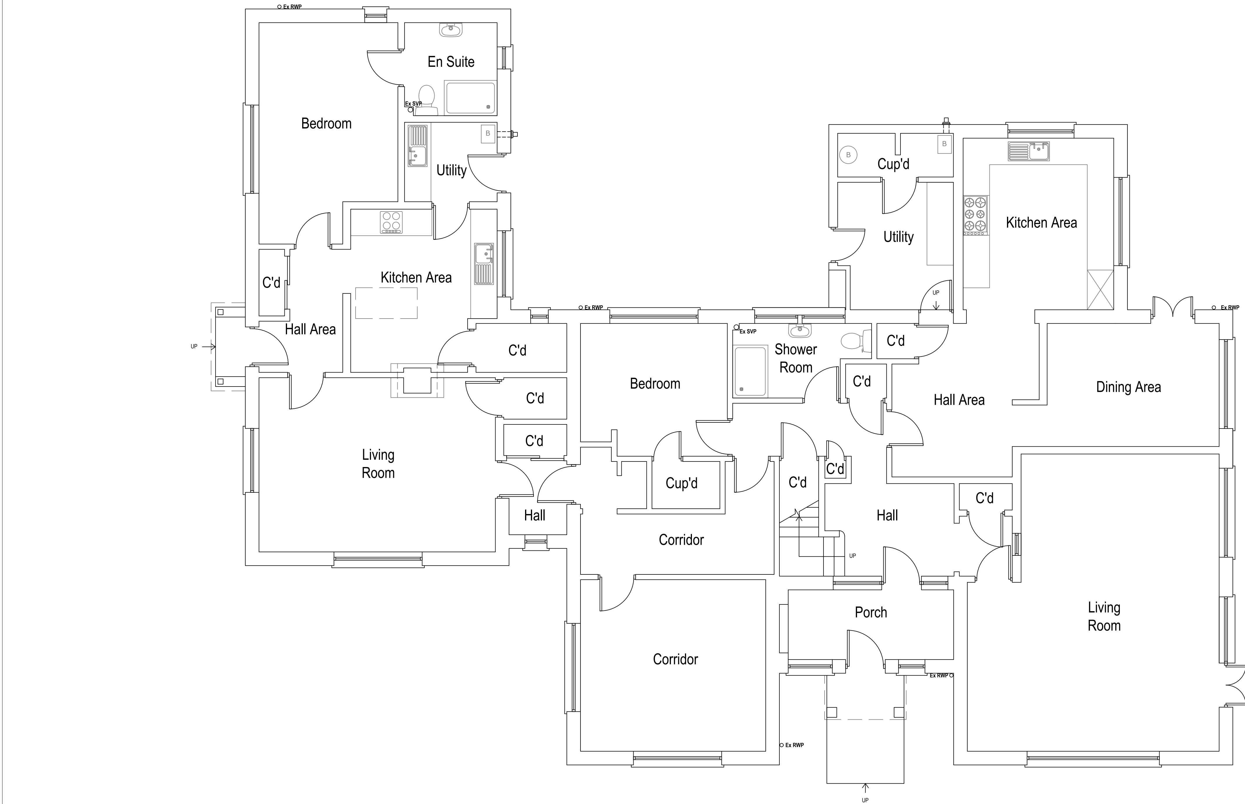
Existing Ground Floor Plan Area ca. 231.01 m 2
