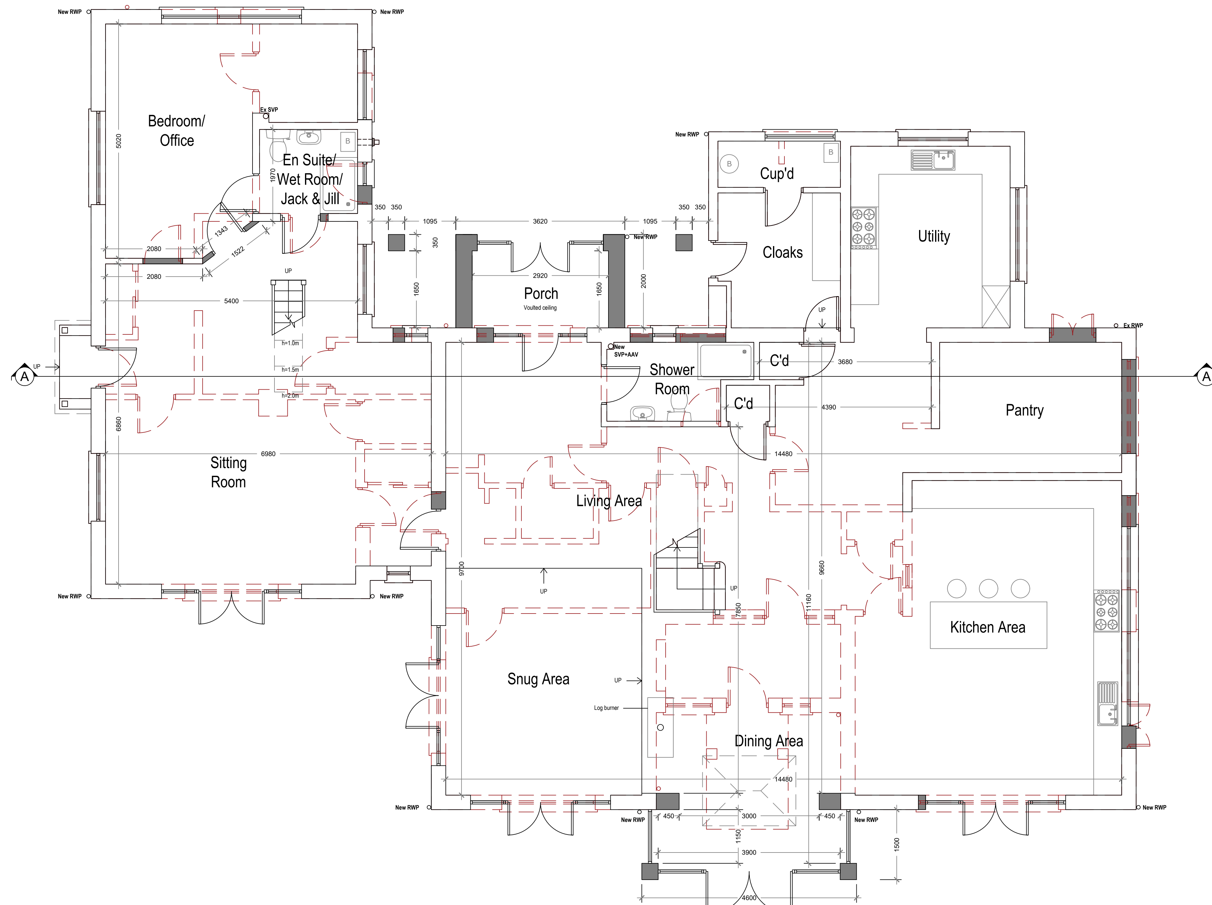
Proposed Ground Floor Plan Area ca. 251.90 m 2
