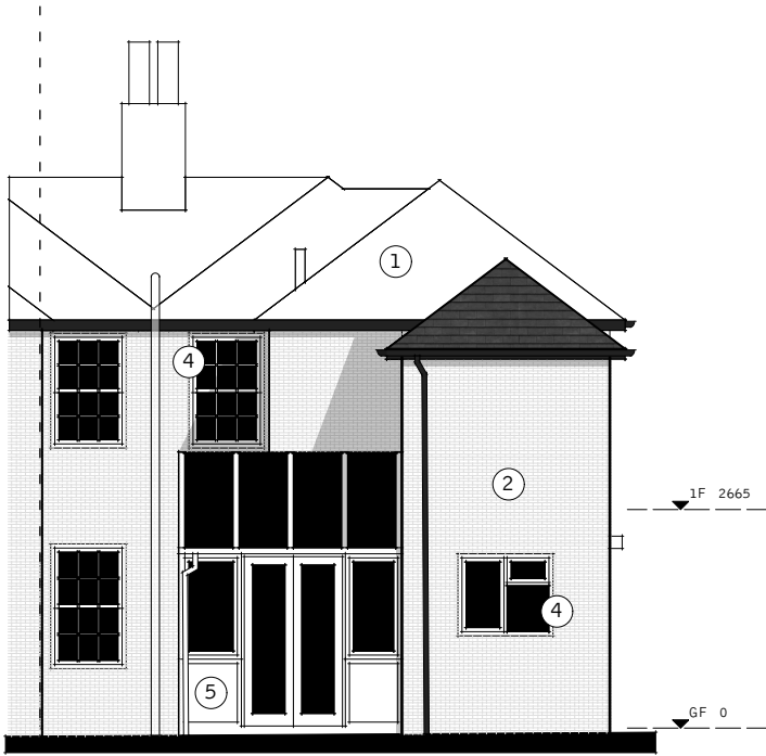
1 North facing elevation Scale: 1:100
