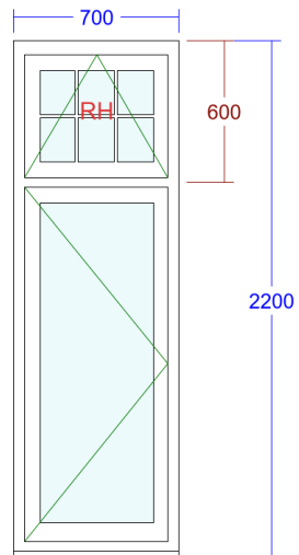
4. Deco Casement Window
