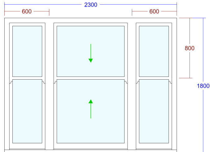
2. Sash Window (LARGE BED SASH)
