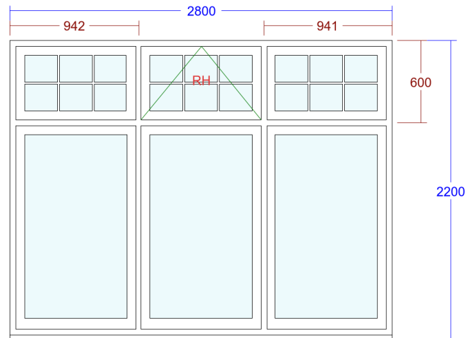
5. Deco Casement Window
