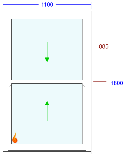
1. Sash Window (SMALL BED SASH)
