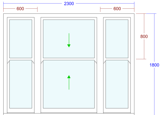
2. Sash Window (LARGE BED SASH)
