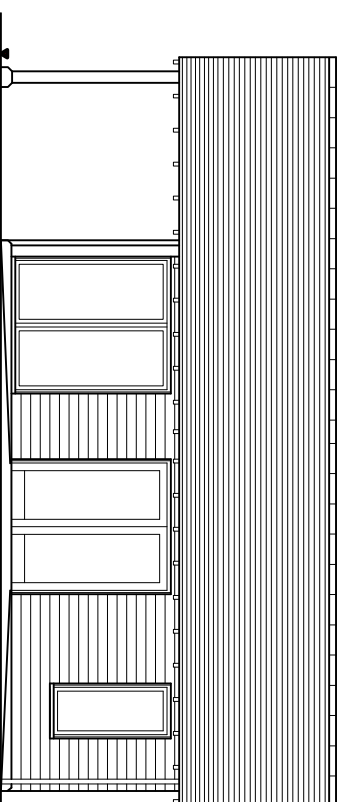
existing east elevation
