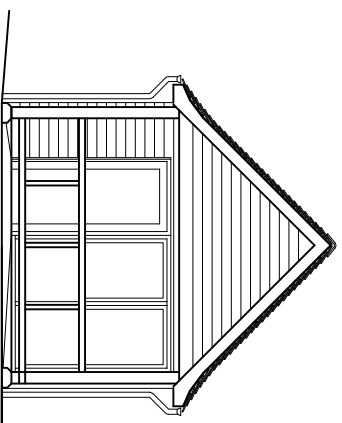
existing south elevation
