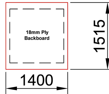
ENCLOSURE REAR VIEW 4
