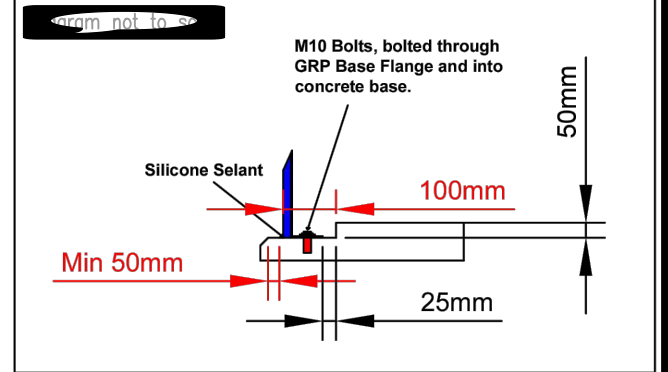
Typical Stepped Concrete Base Detail (Recommended)
