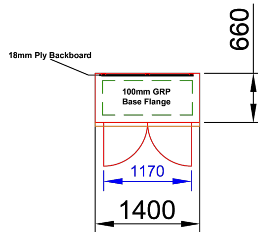
ENCLOSURE PLAN VIEW 1
