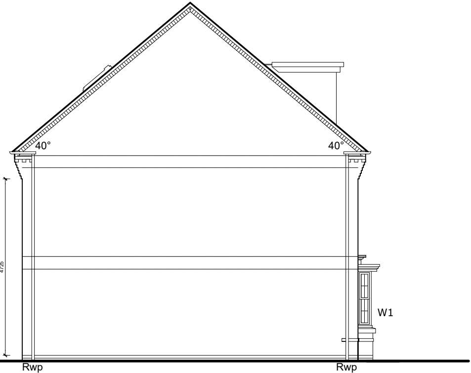
SIDE ELEVATION
