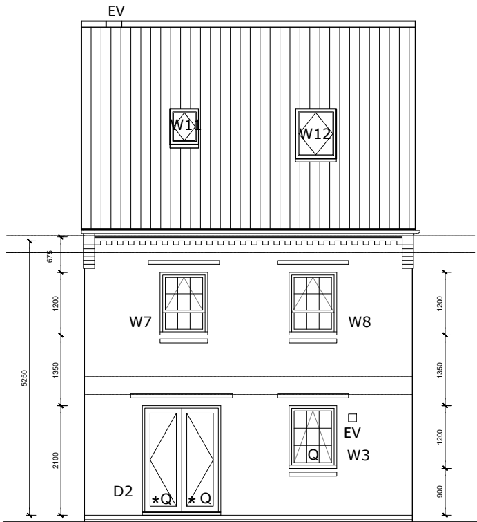
REAR ELEVATION
