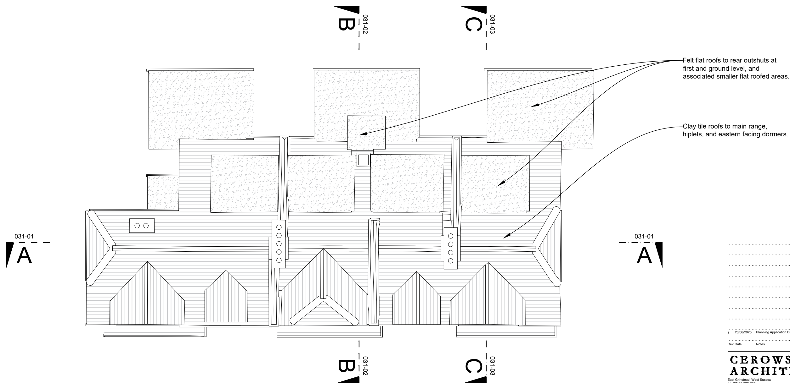
1 Roof Plan Existing 1:100 Scale in metres 0 0.5 1.0 2.0 3.0 4.0 5.0 10.0 N
