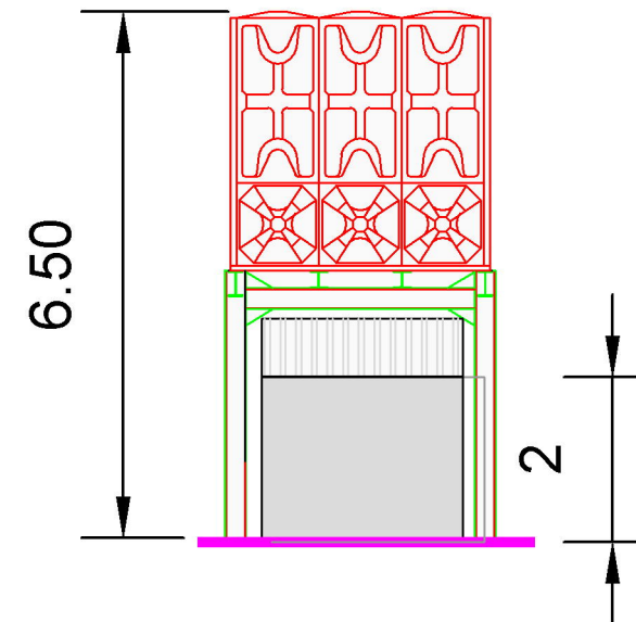
East Elevation
