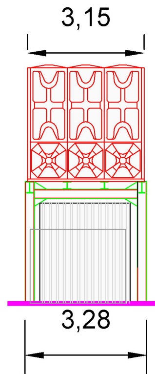
West Elevation
