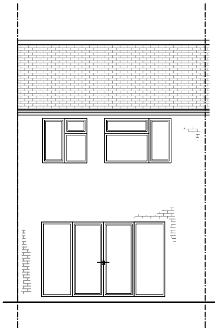
Existing Rear Elevation Scale 1/100@A3
