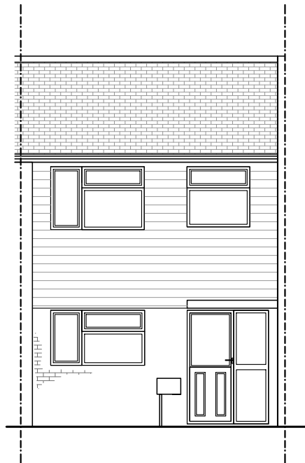
Existing Front Elevation Scale 1/100@A3
