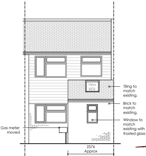
Proposed Front Elevation Scale 1/100@A3
