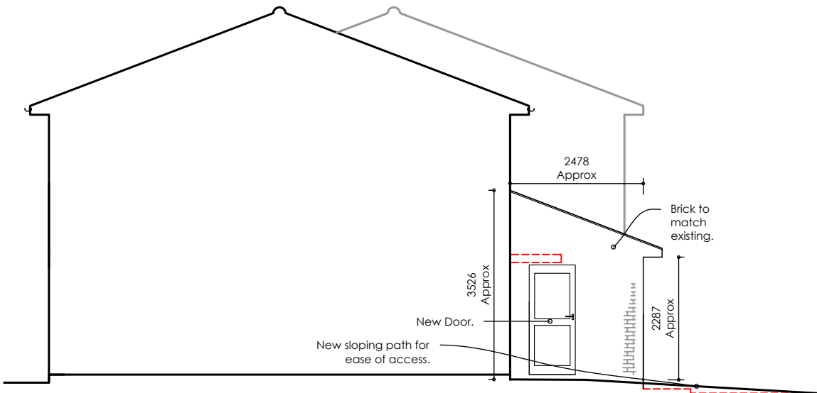
Proposed LHS Elevation Scale 1/100@A3
