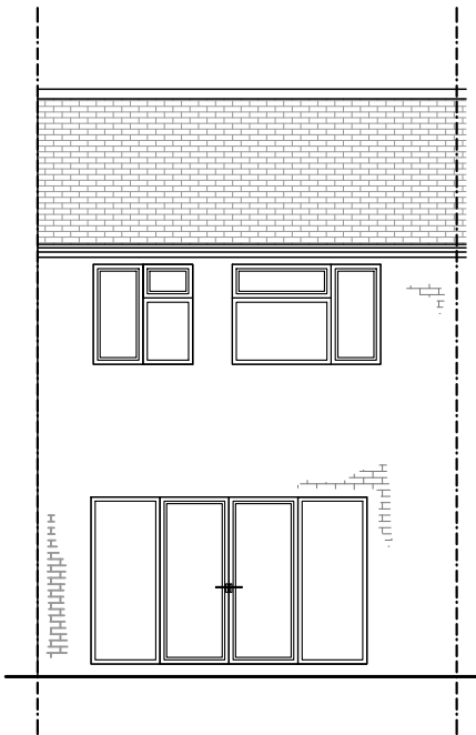
Proposed Rear Elevation Scale 1/100@A3
