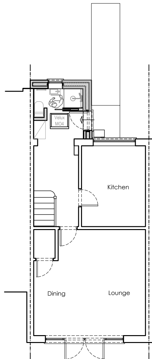
Proposed Ground Floor Plan Scale 1/100@A3
