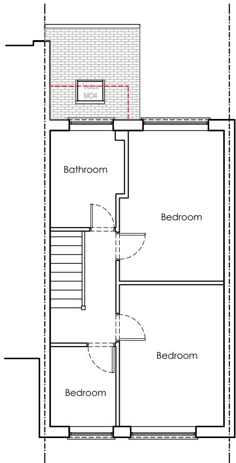
Proposed First Floor Plan Scale 1/100@A3
