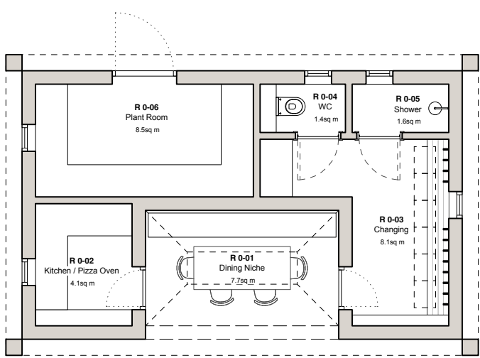
A Pool Pavilion - Ground Floor Plan Scale: 1:100
