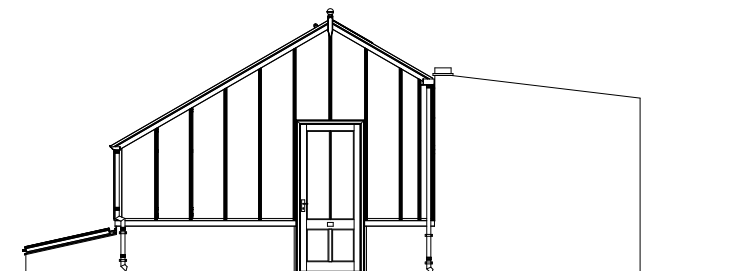
6 Glasshouse - East Elevation Scale: 1:100
