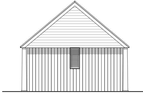
3 Pool Pavilion - East Elevation Scale: 1:100
