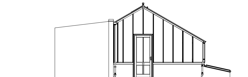
5 Glasshouse - West Elevation Scale: 1:100
