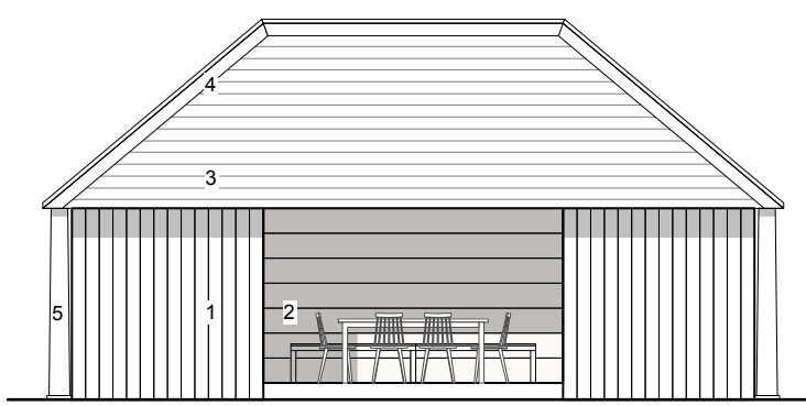
1 Pool Pavilion - South Elevation Scale: 1:100
