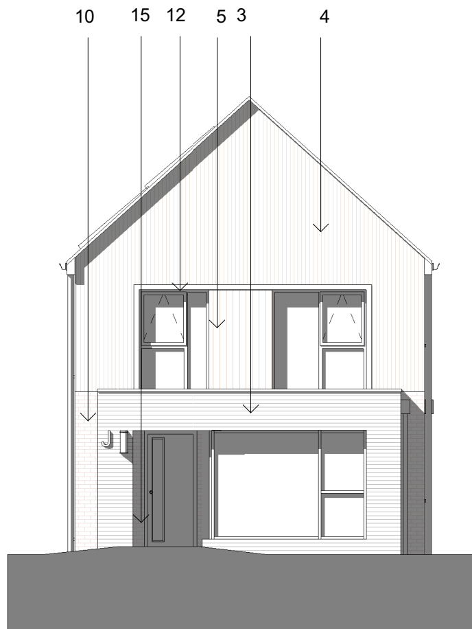
Front Elevation 1 : 100
