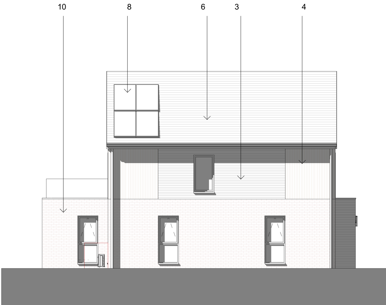
Side Elevation 1 1 : 100
