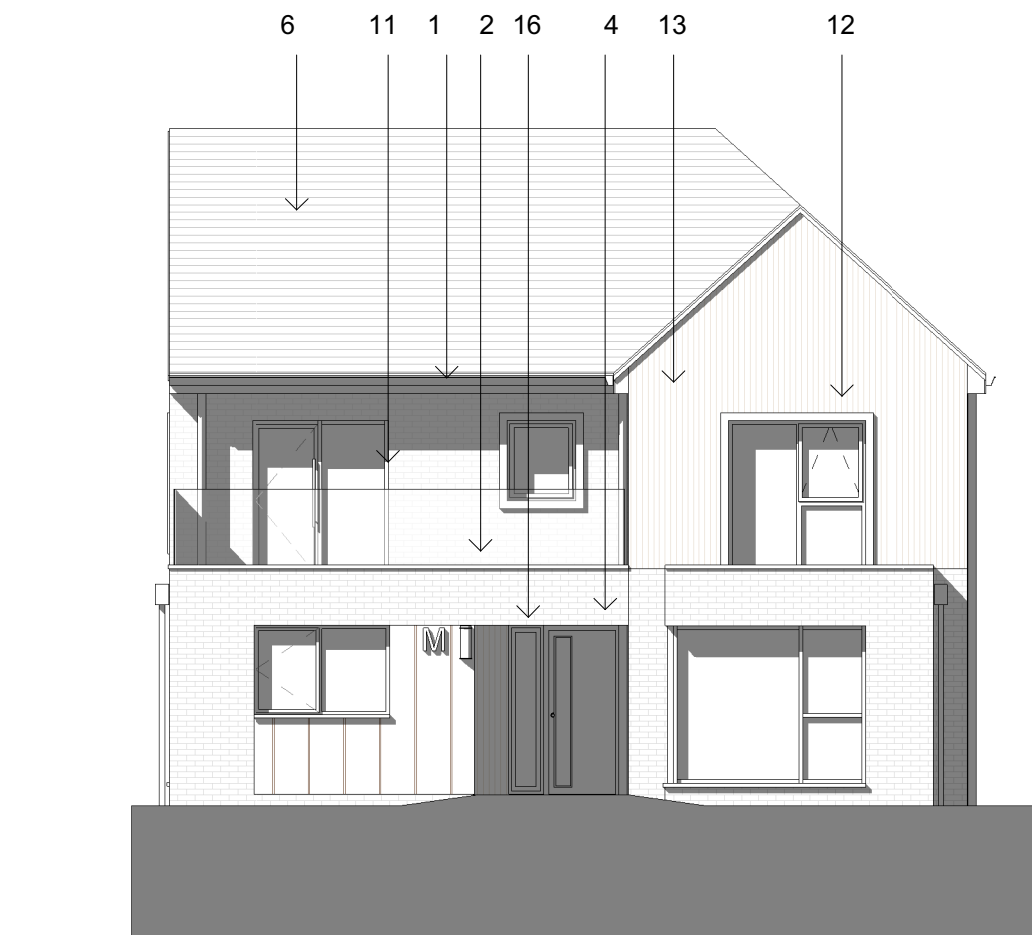
Front Elevation 01 1 : 100
