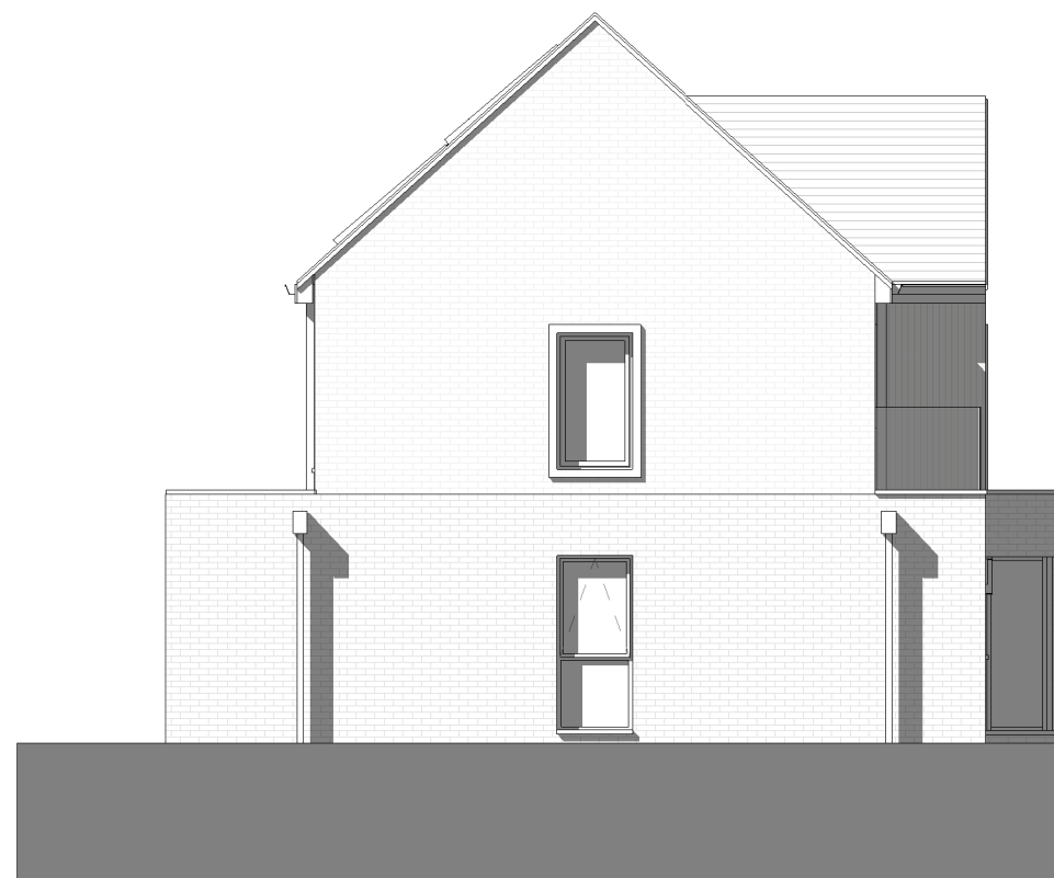
Side Elevation 2 1 : 100
