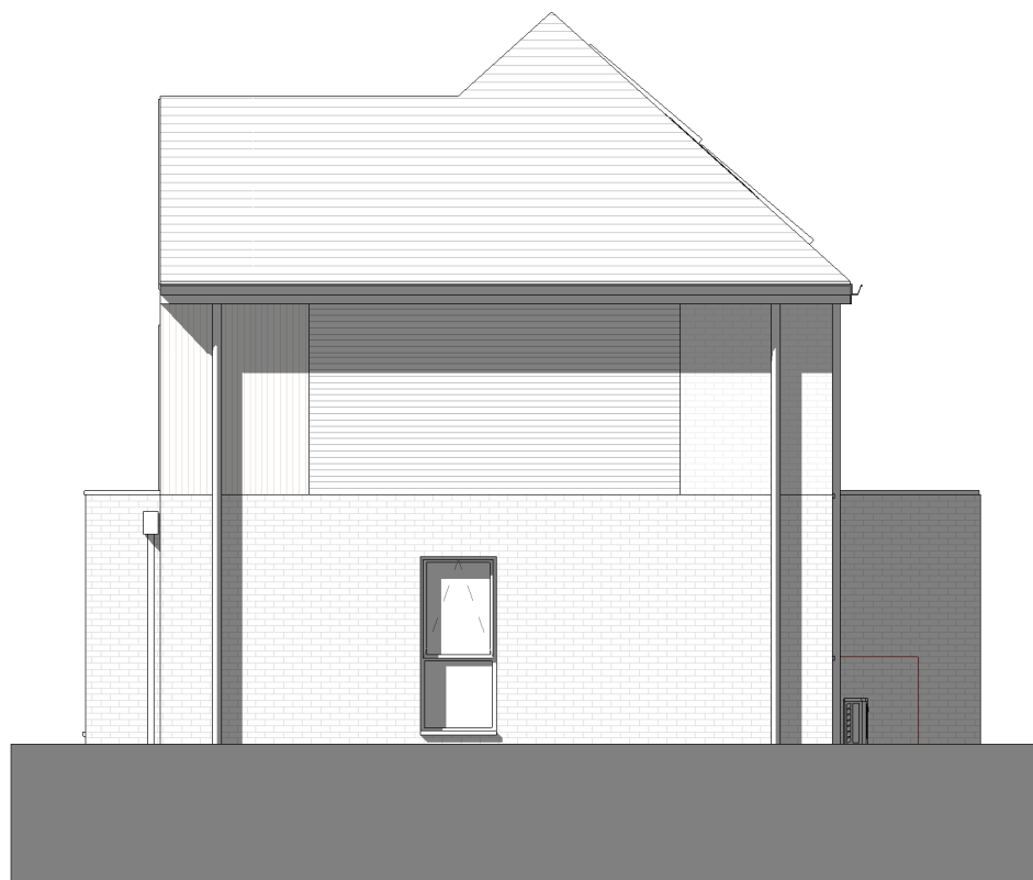
Side Elevation 1 1 : 100
