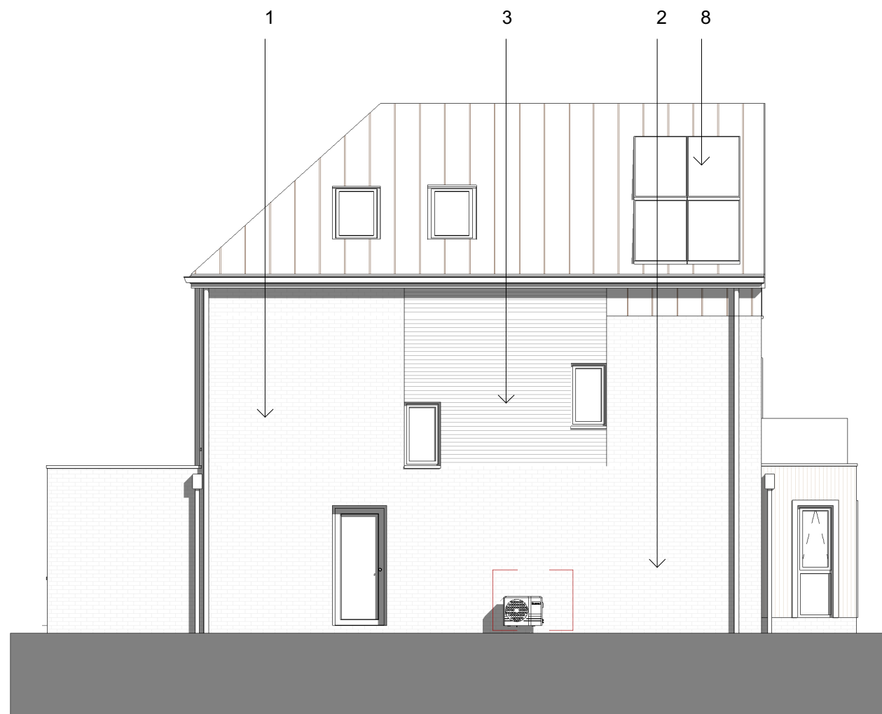
Side Elevation 1 1 : 100
